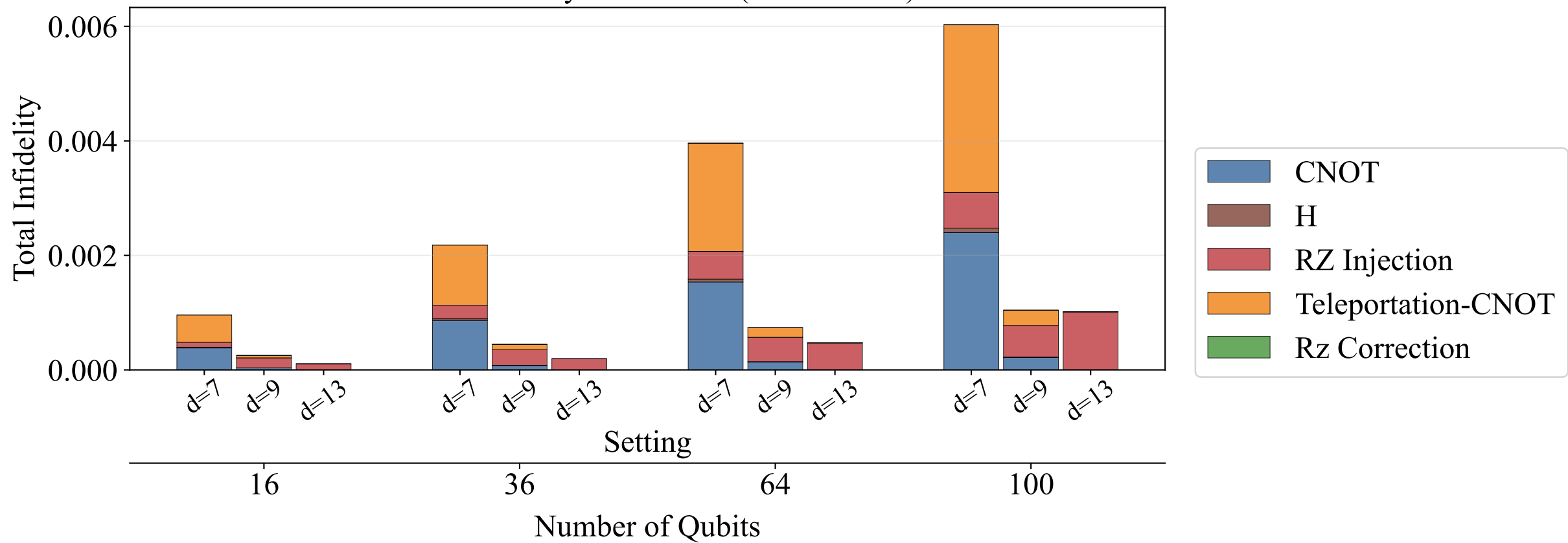
STAR Infidelity Breakdown (Without Idle)
