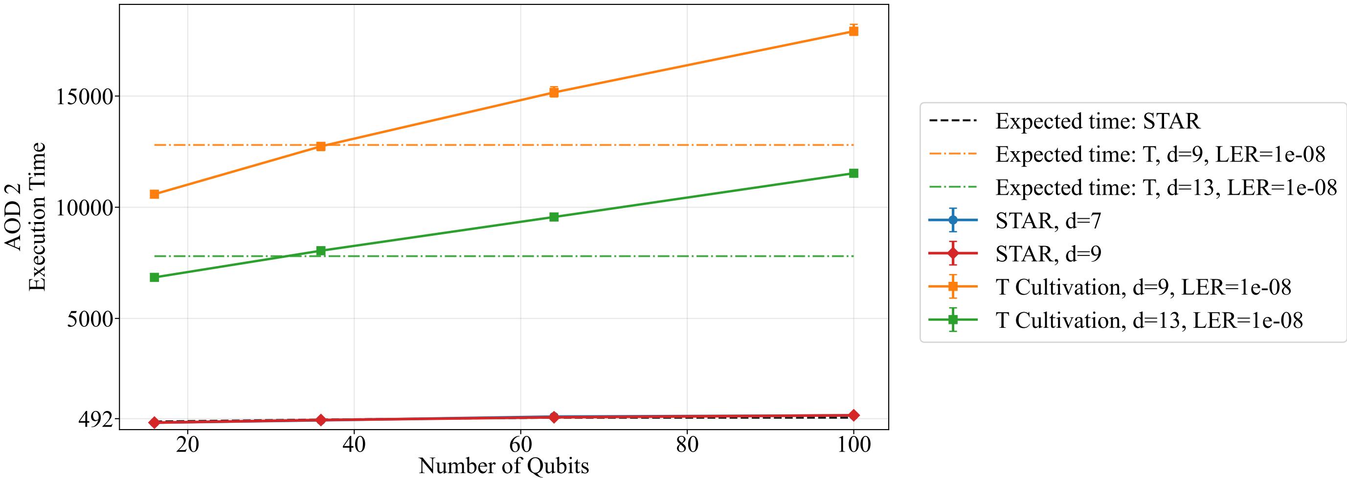
STAR vs T cultivation runtime One Trotter Step
