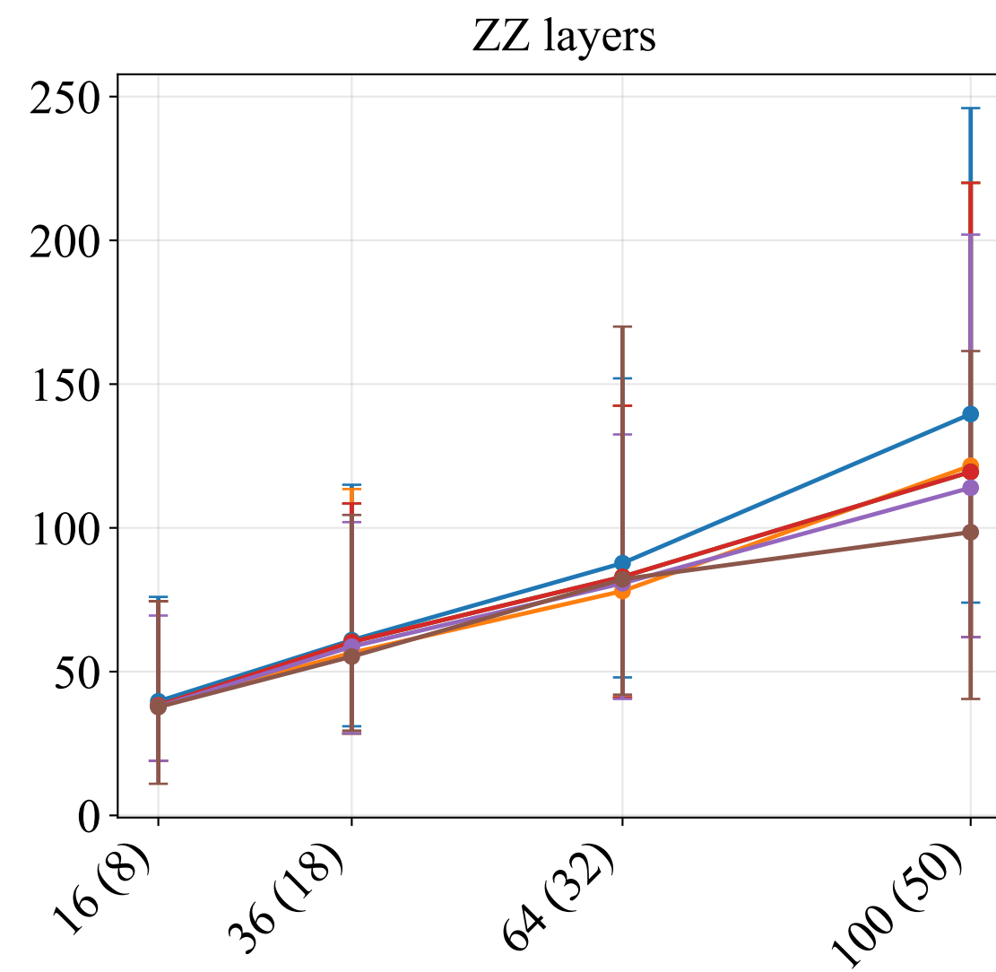
Ablation Study, Execution Time, distance=13
