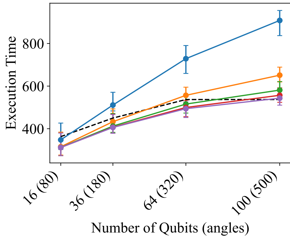
Full Trotter
