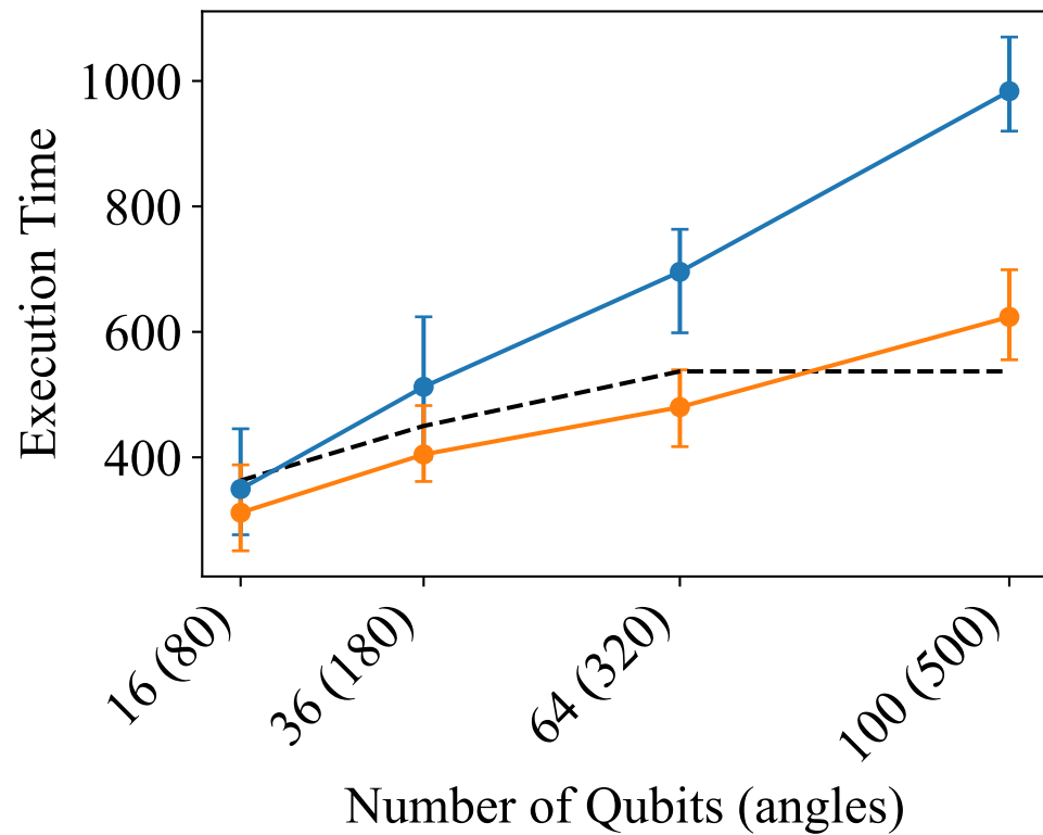
Full Trotter
