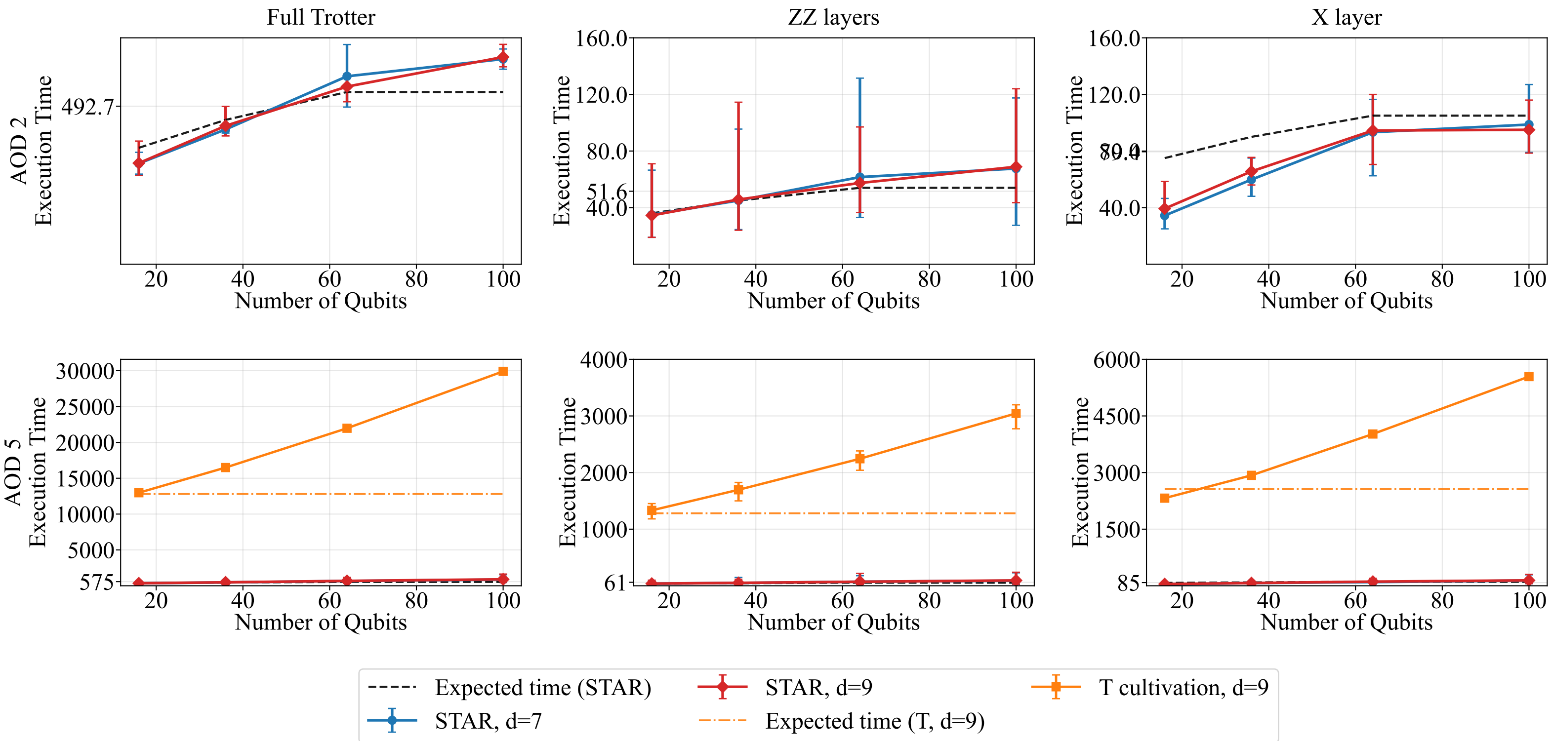
STAR vs T cultivation runtime · Columns: Full Trotter | ZZ layers | X layer · Rows: AOD 2 (top), AOD 5 (bottom) · T: Seperate Row Region
