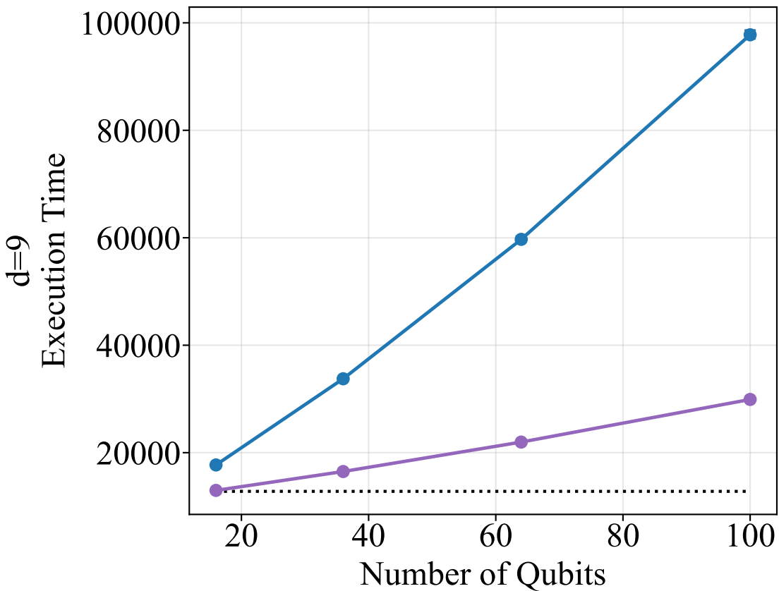
Full Trotter
