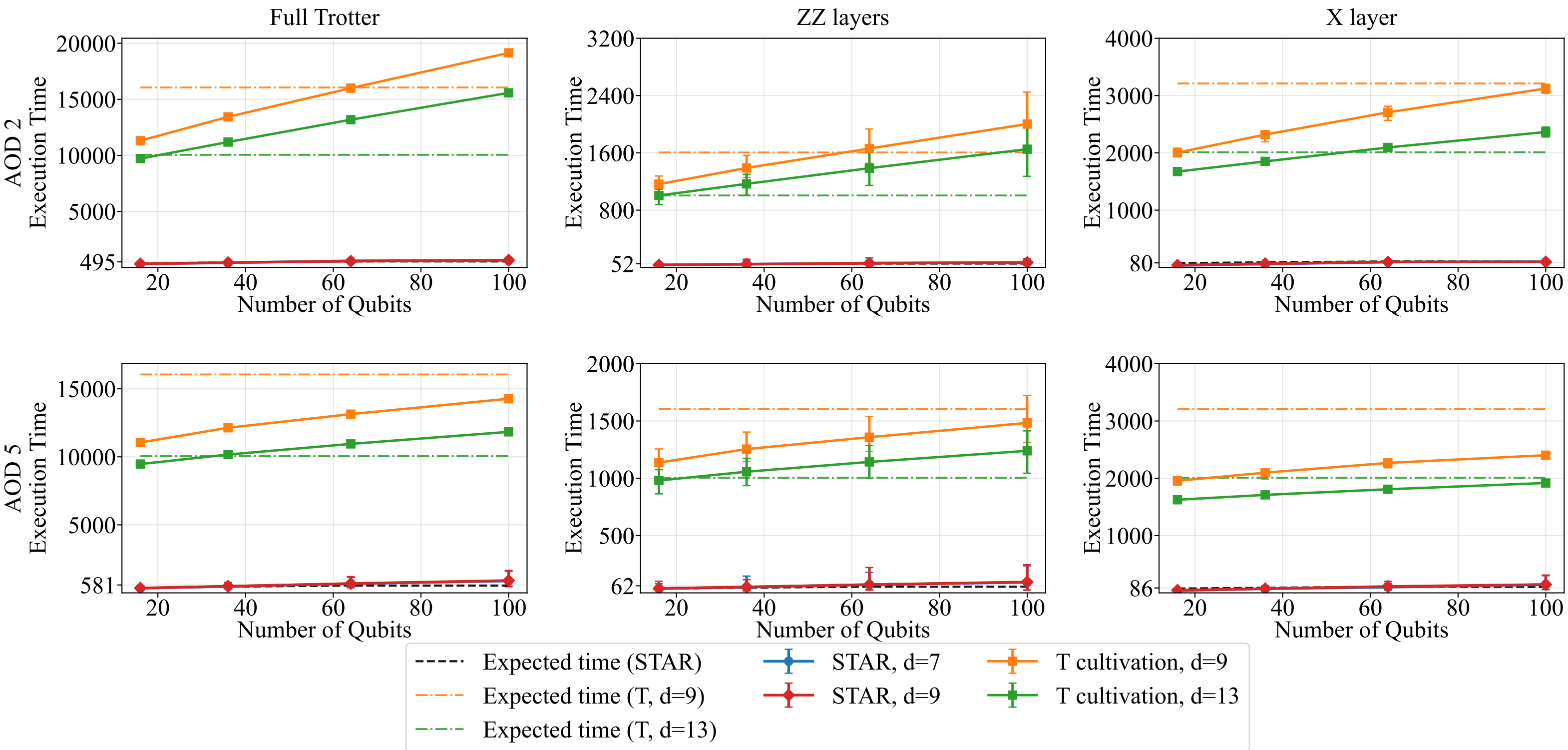
STAR vs T cultivation runtime · Columns: Full Trotter | ZZ layers | X layer · Rows: AOD 2 (top), AOD 5 (bottom) · T: Column-Based
