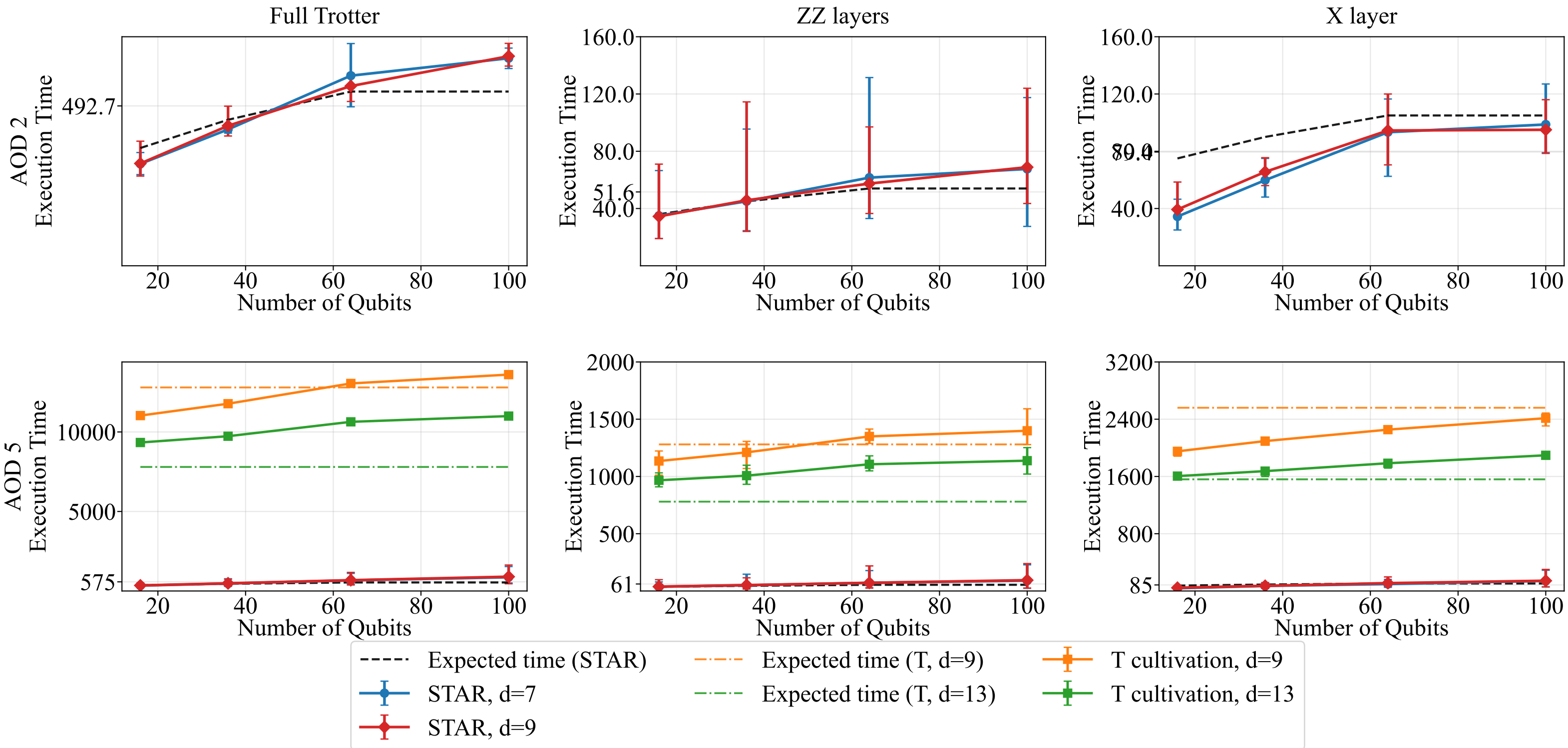
STAR vs T cultivation runtime · Columns: Full Trotter | ZZ layers | X layer · Rows: AOD 2 (top), AOD 5 (bottom) · T: Checkerboard
