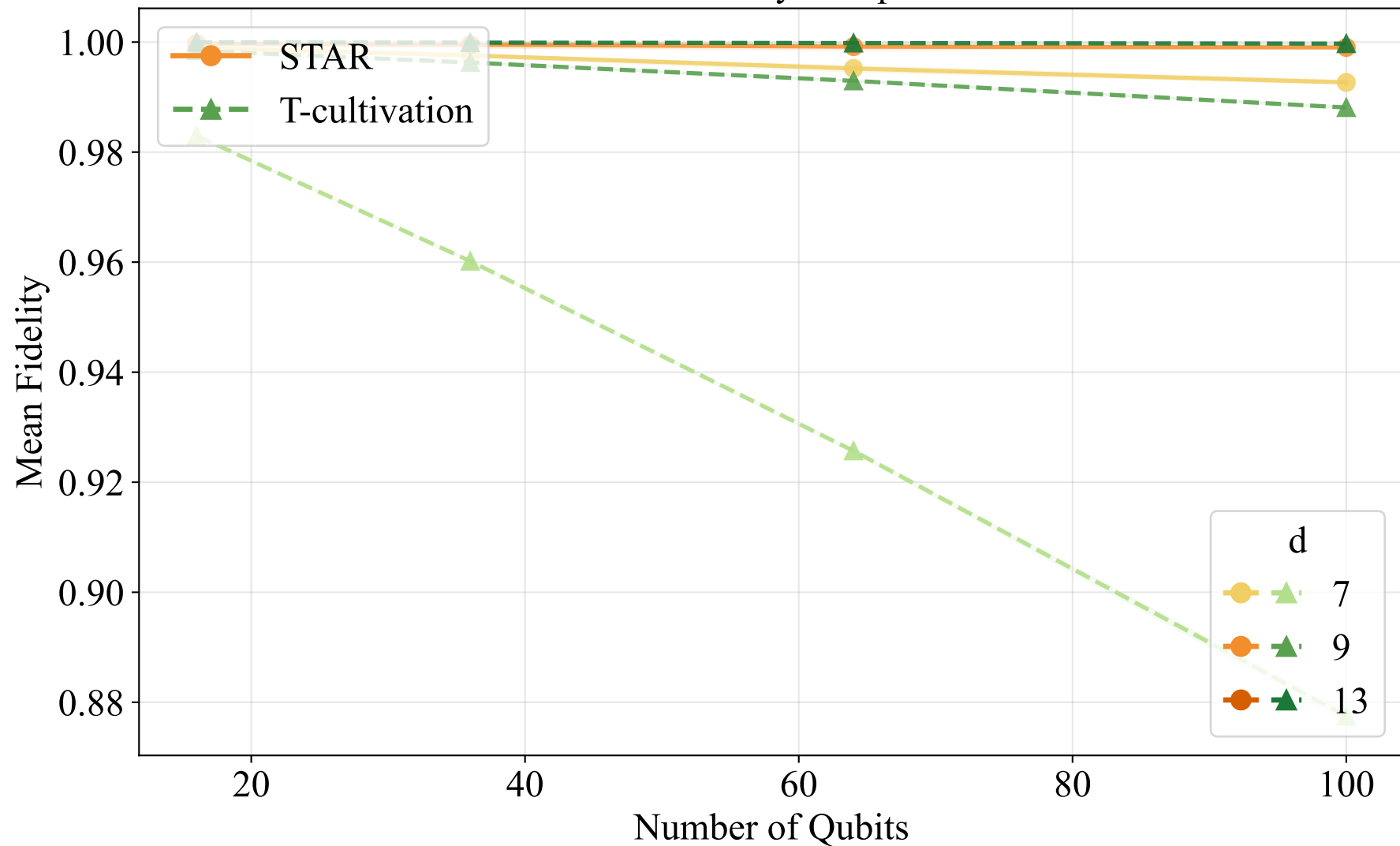
Overall Fidelity Comparison
