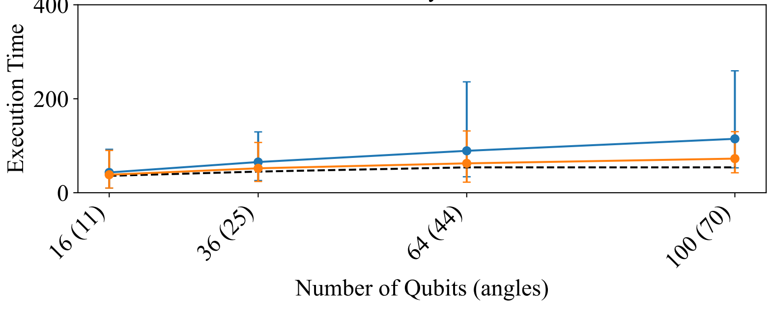
ZZ layers
