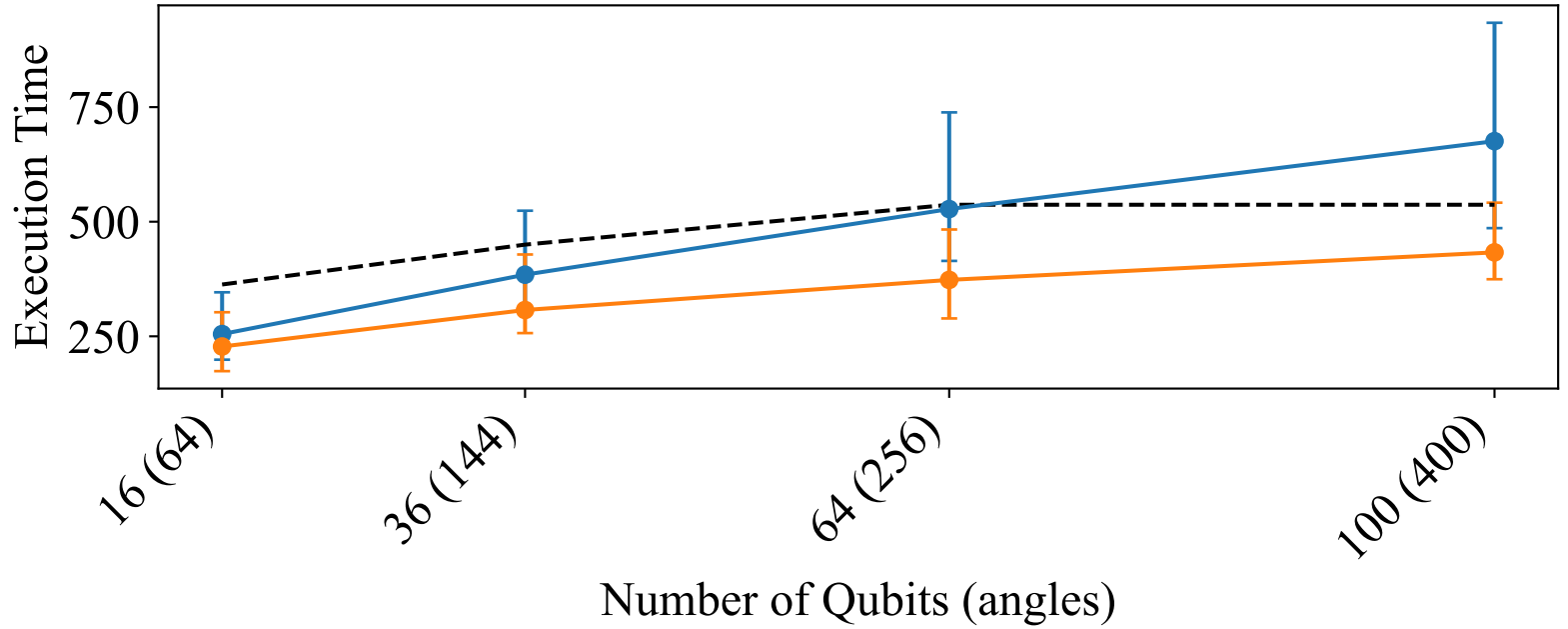
Full Trotter
