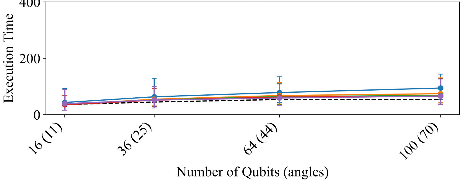
ZZ layers
