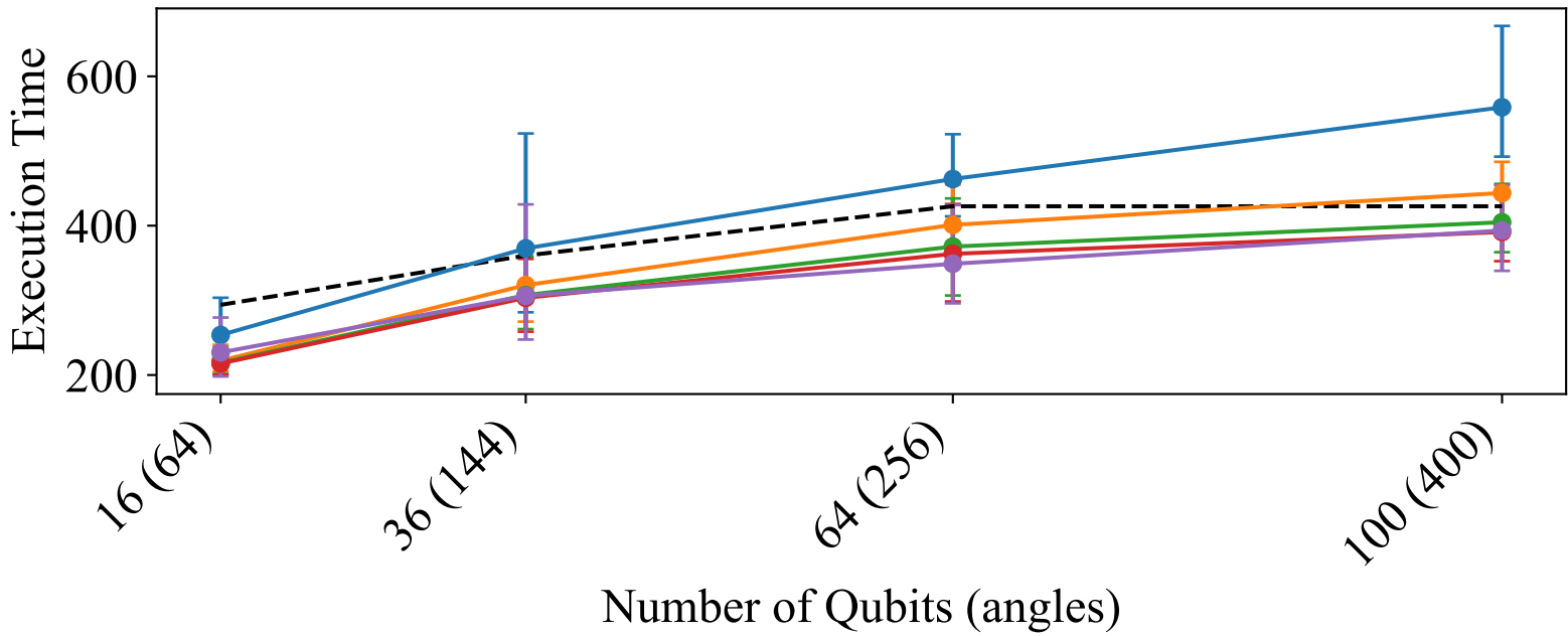
Full Trotter
