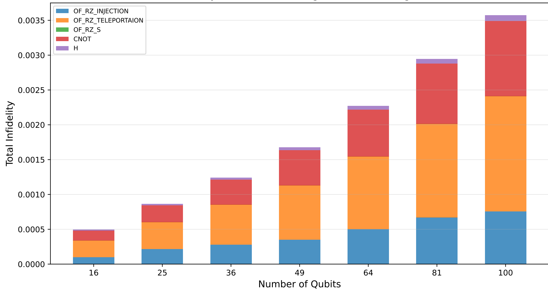
STAR Infidelity Breakdown (Averaged Over All Configurations)
