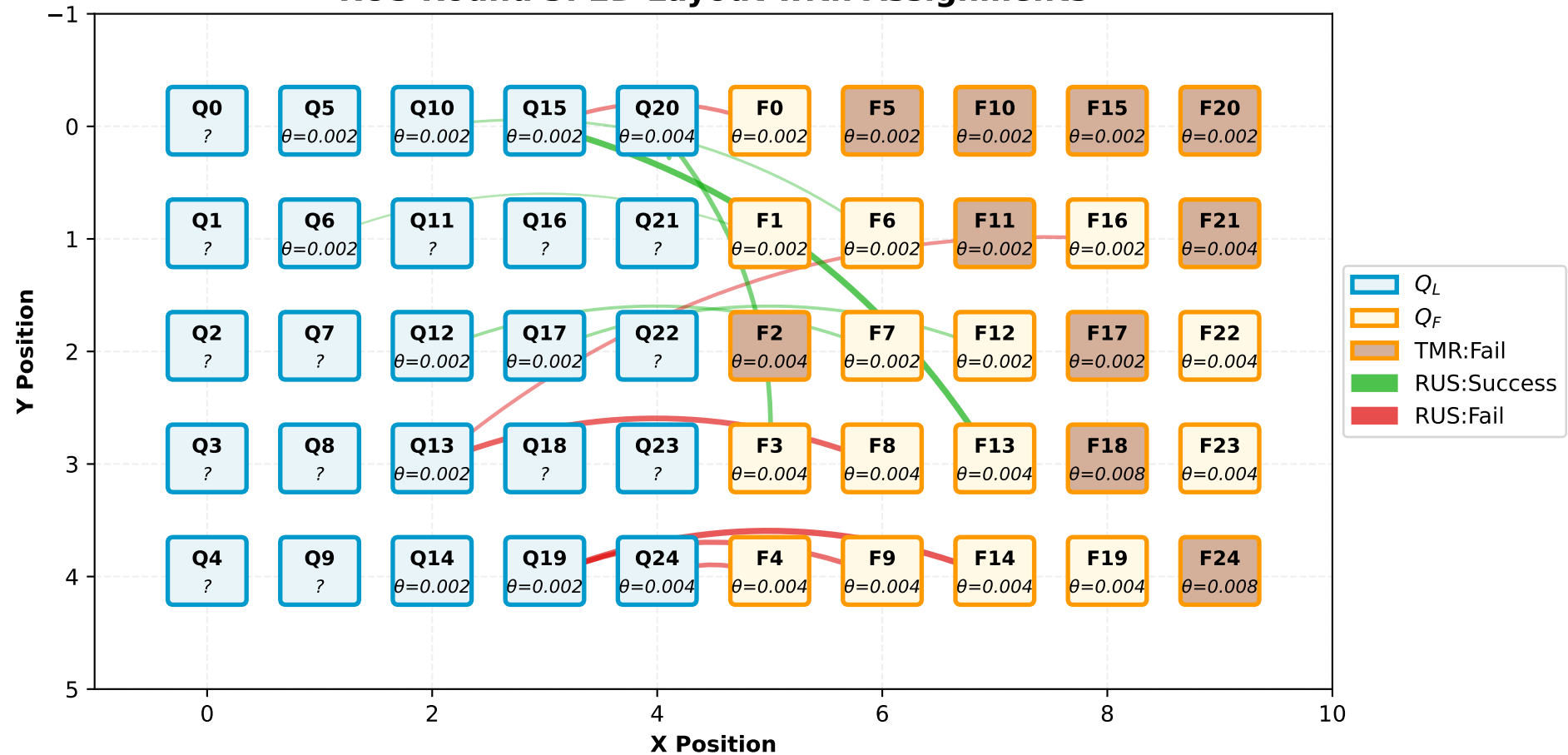
RUS Round 3: 2D Layout with Assignments
