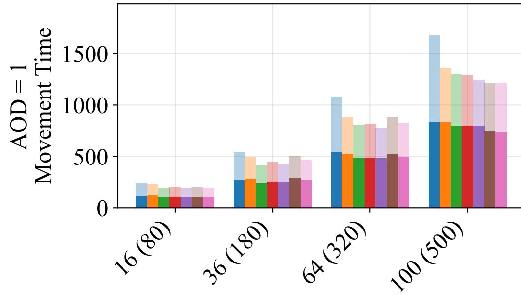
Full Trotter
