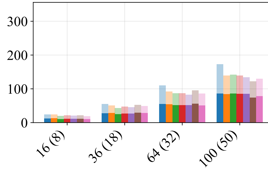
ZZ layers
