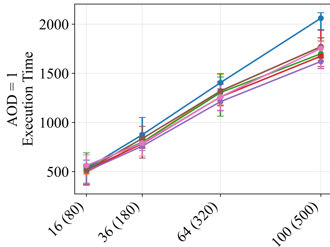
Full Trotter
