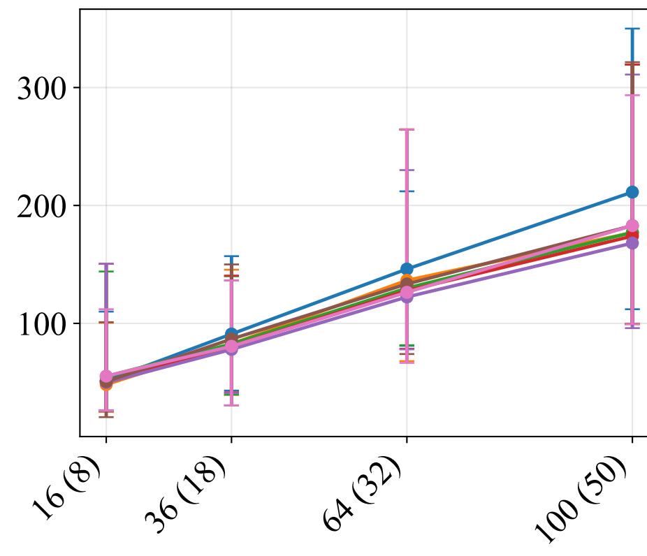
ZZ layers
