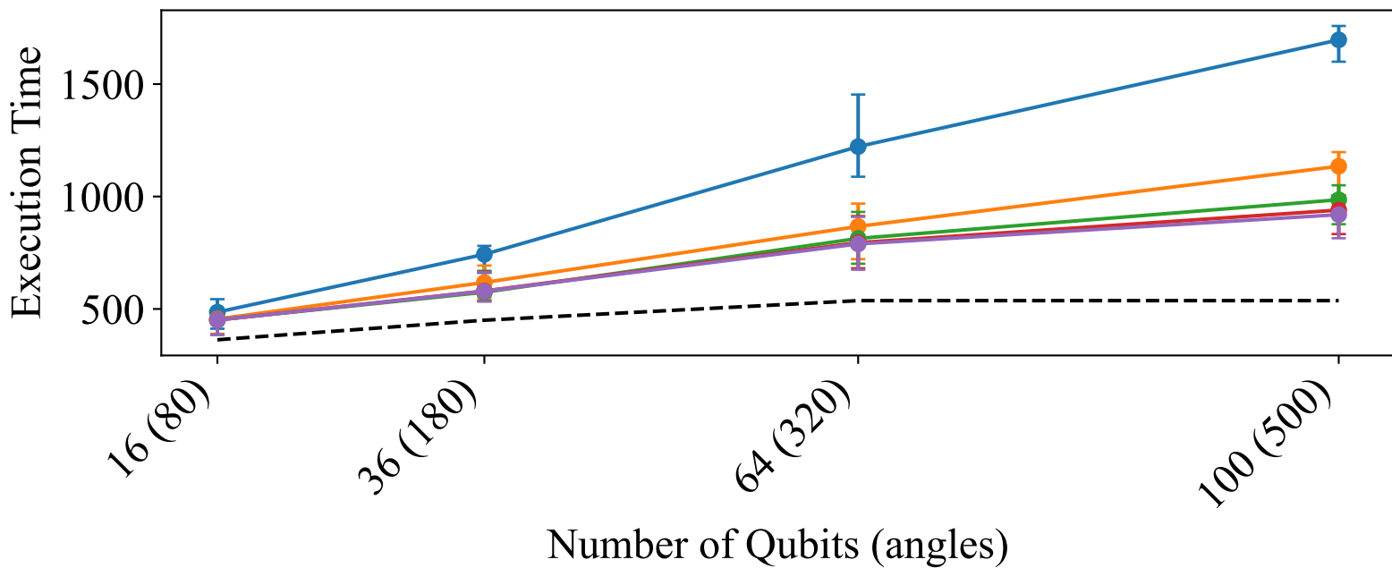
Full Trotter
