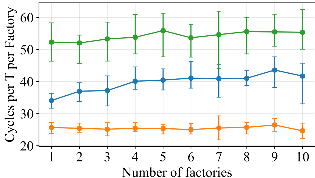
Comparison: Number of Factories < Number of Qubits (10 qubits, each with 10 T gates)
