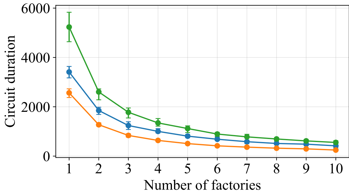
Comparison: Number of Factories < Number of Qubits (10 qubits, each with 10 T gates)
