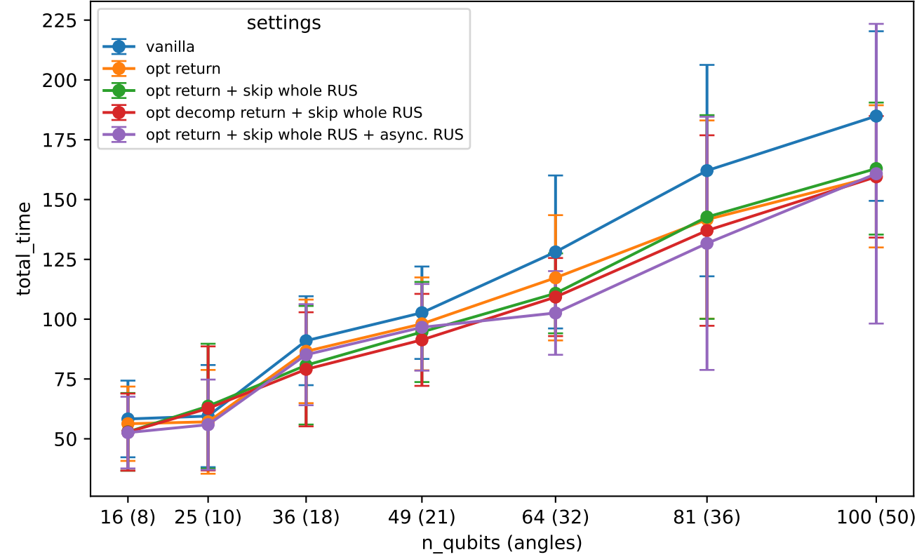
Ablation Study: Total Execution Time - round_1
