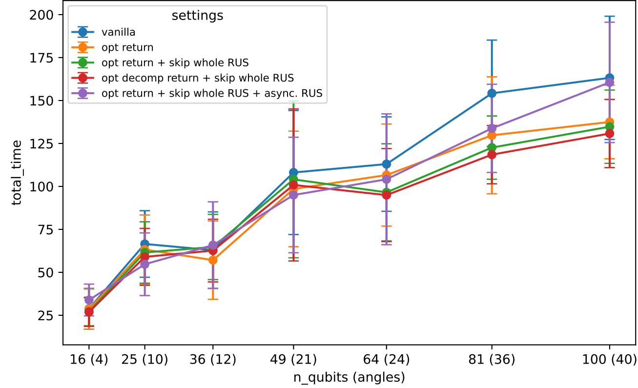
Ablation Study: Total Execution Time - round_2
