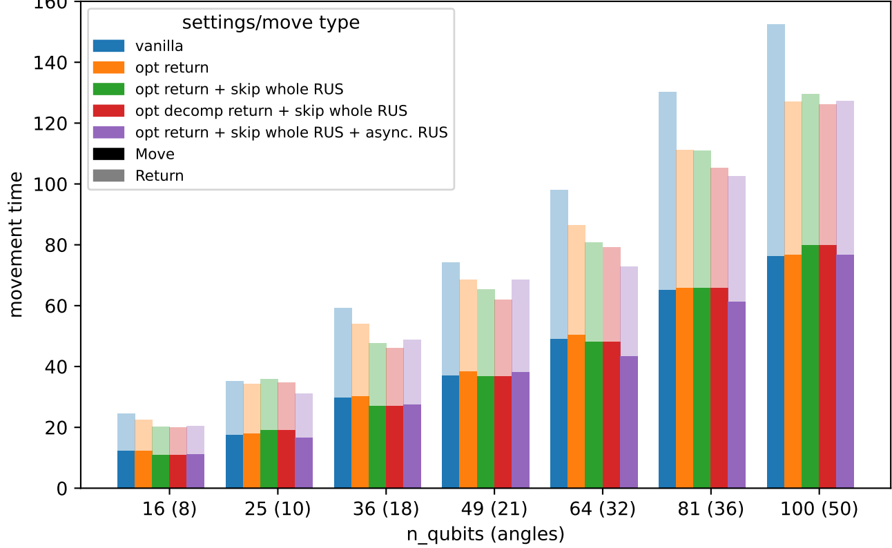
Ablation Study: Movement Time Breakdown - round_1
