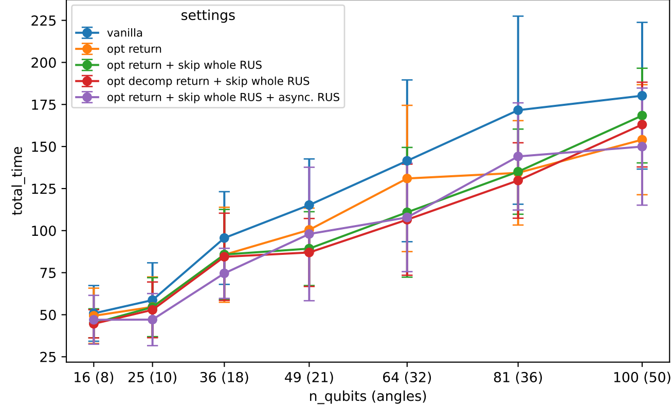
Ablation Study: Total Execution Time - round_3
