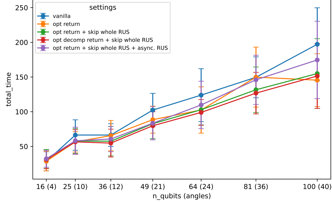
Ablation Study: Total Execution Time - round_4
