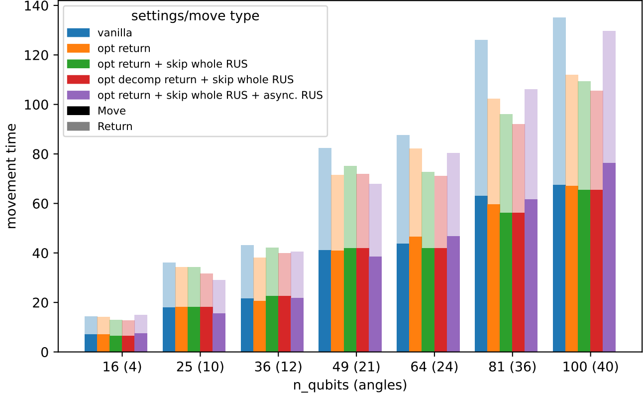
Ablation Study: Movement Time Breakdown - round_2
