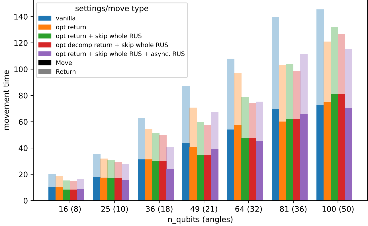
Ablation Study: Movement Time Breakdown - round_3
