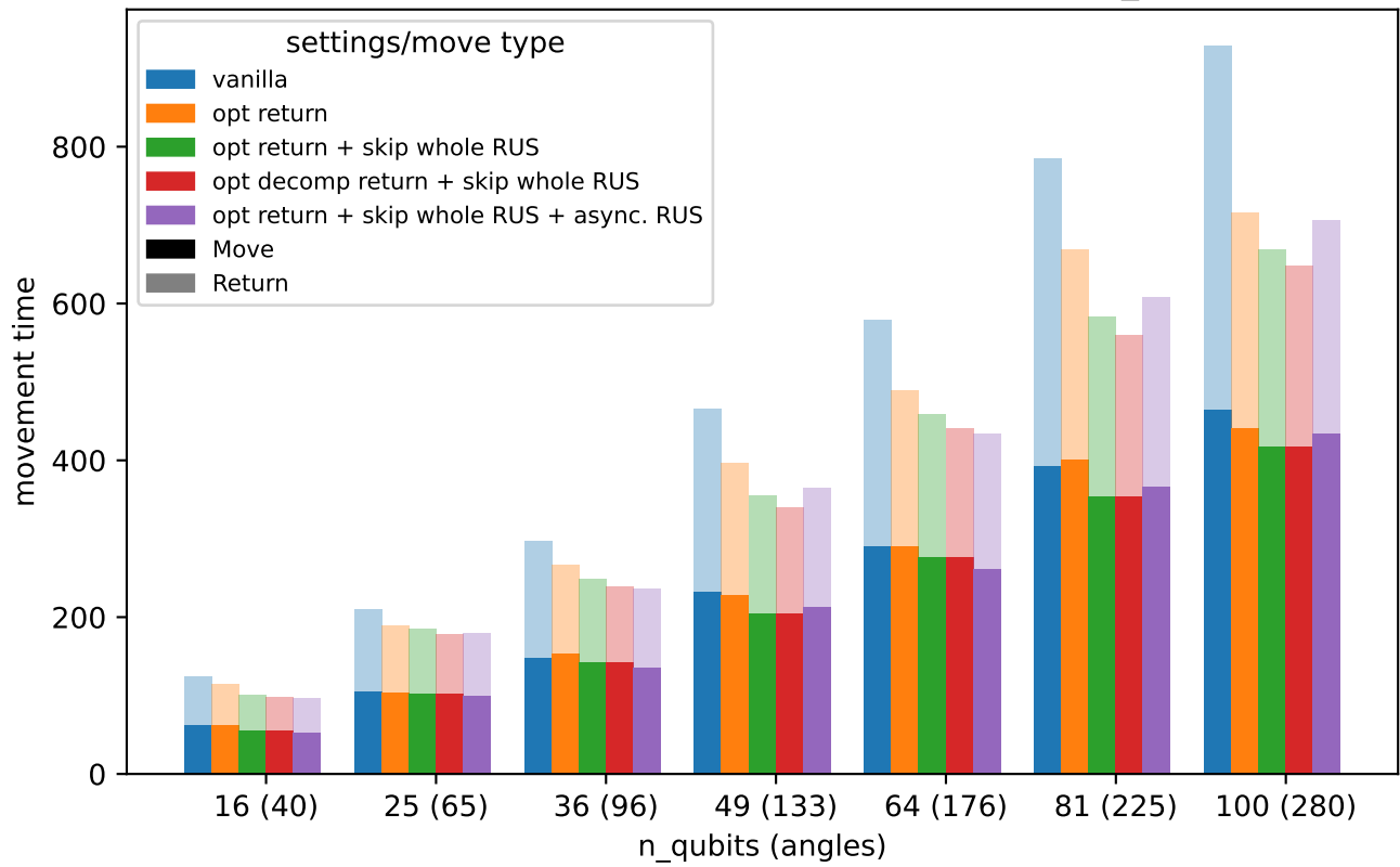
Ablation Study: Movement Time Breakdown - round_0
