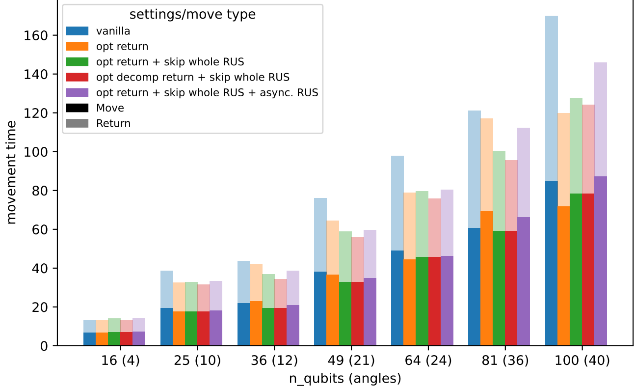
Ablation Study: Movement Time Breakdown - round_4
