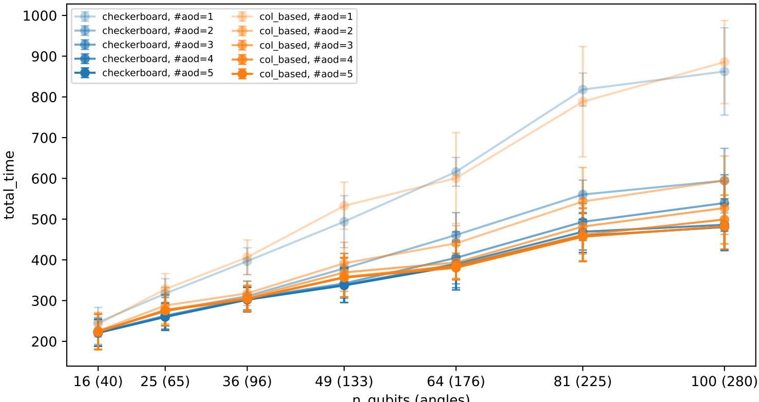
Total time for placement \times #aod - round_0
