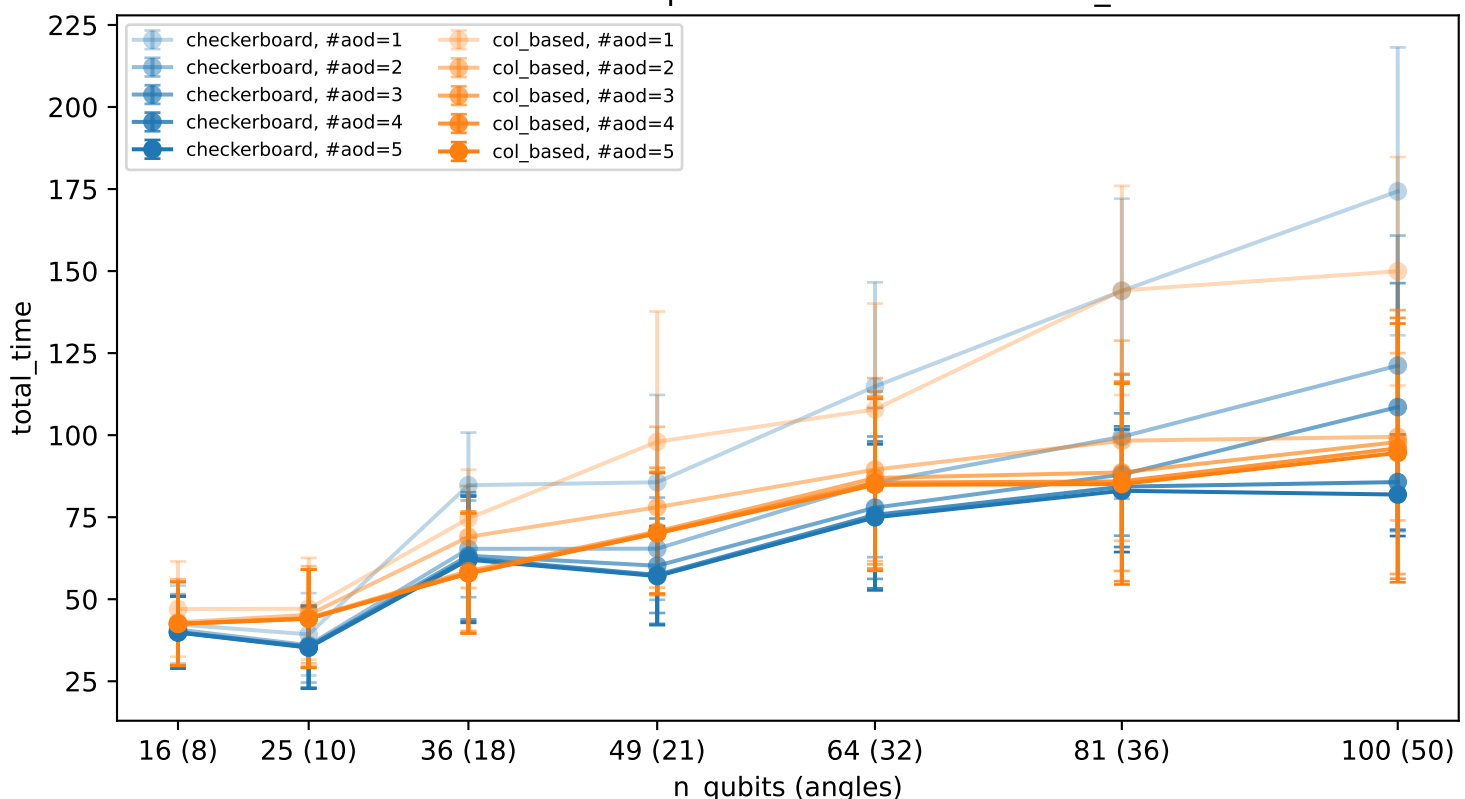
Total time for placement \times #aod - round_3
