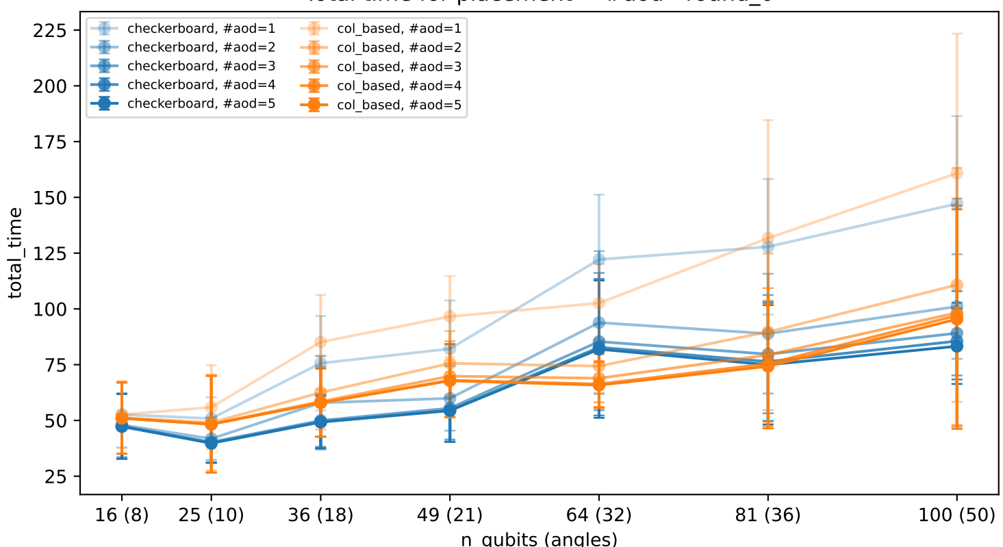
Total time for placement \times #aod - round_1
