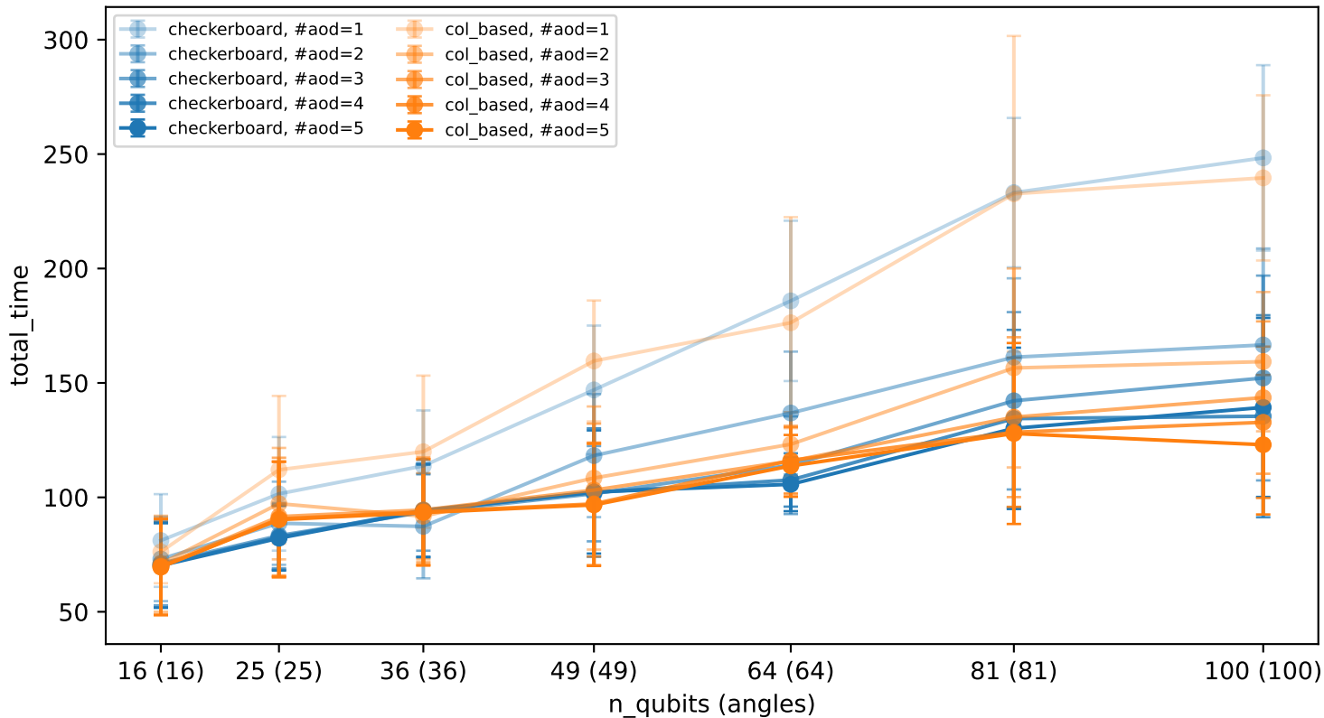
Total time for placement \times #aod - round_4
