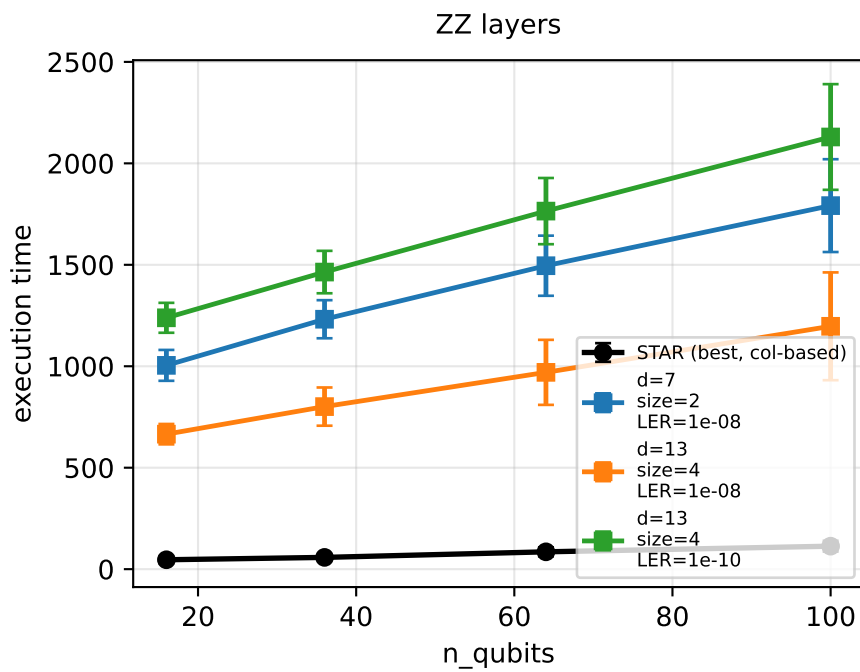
STAR vs T cultivation (STAR code distance = 7) · Columns: Full trotter | ZZ layers | X layer · Rows: AOD 2 (top), AOD 5 (bottom)
