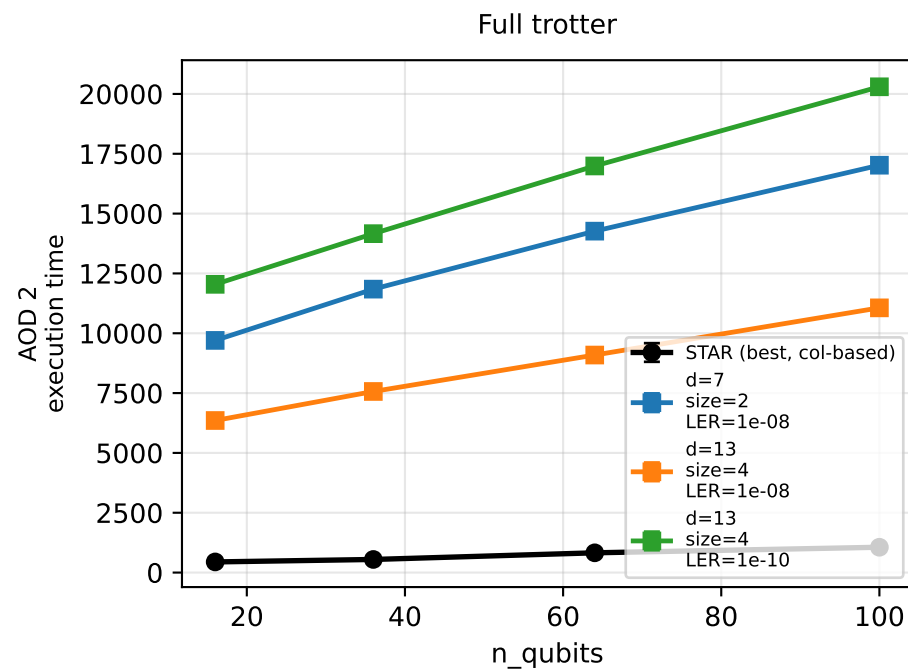
STAR vs T cultivation (STAR code distance = 7) · Columns: Full trotter | ZZ layers | X layer · Rows: AOD 2 (top), AOD 5 (bottom)
