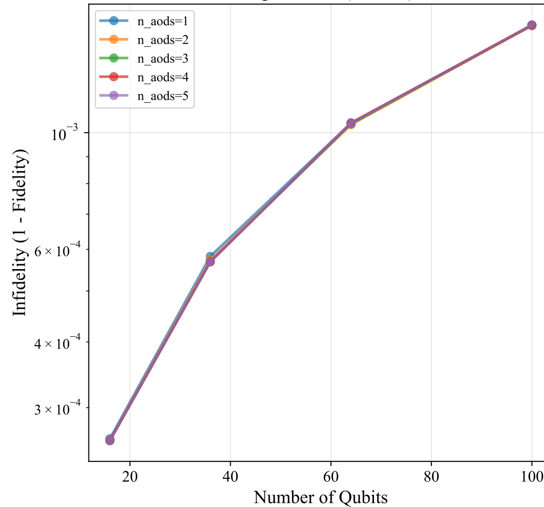
Teleportation (CNOT)
