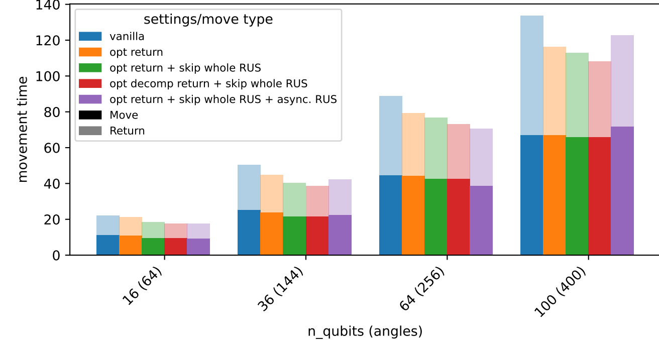
Movement Time Breakdown - X layer
