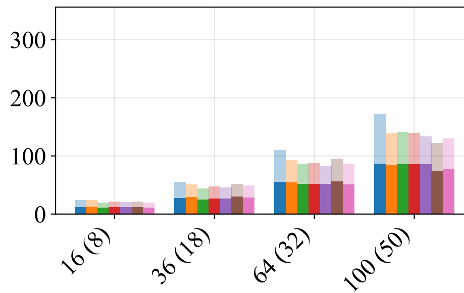
ZZ layers
