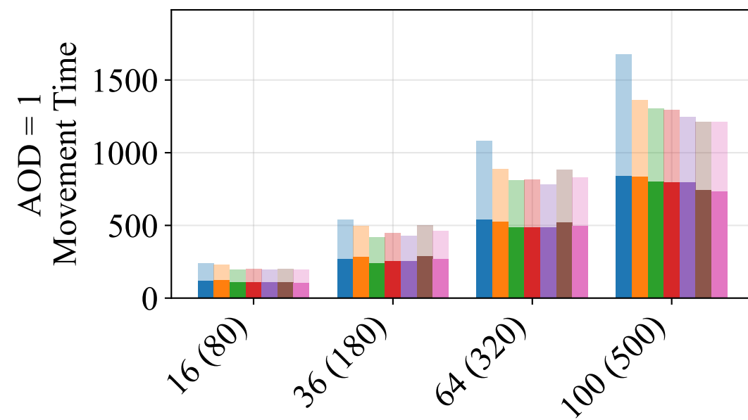
Full Trotter
