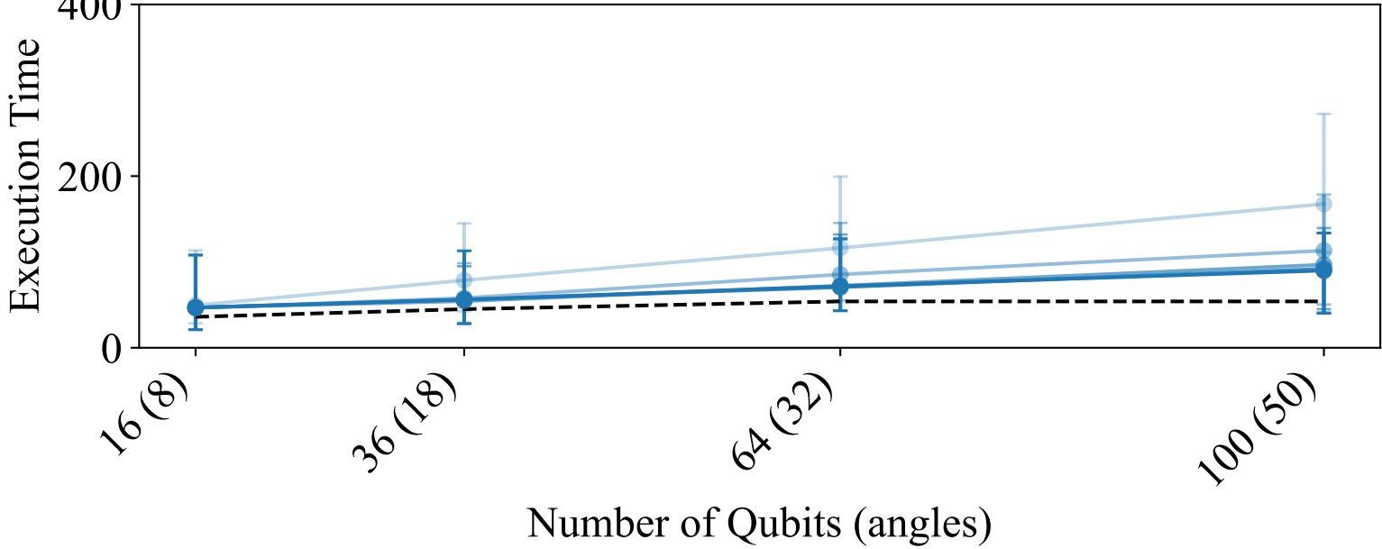
ZZ layers
