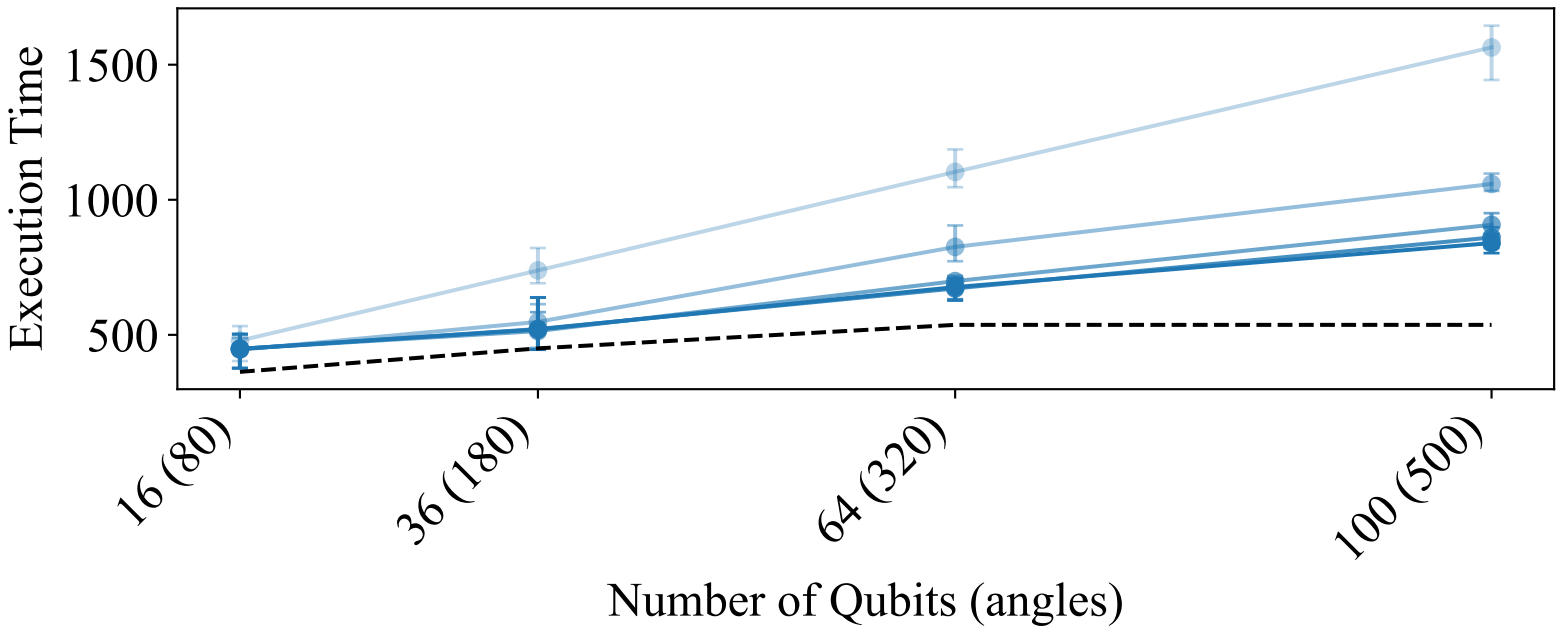
Full Trotter
