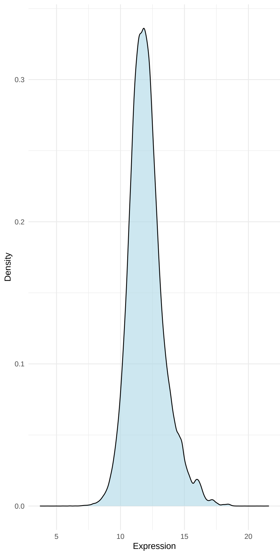
Density Plot of All Log-Intensity Values
