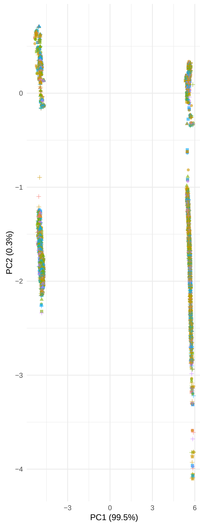
ASCA on day
