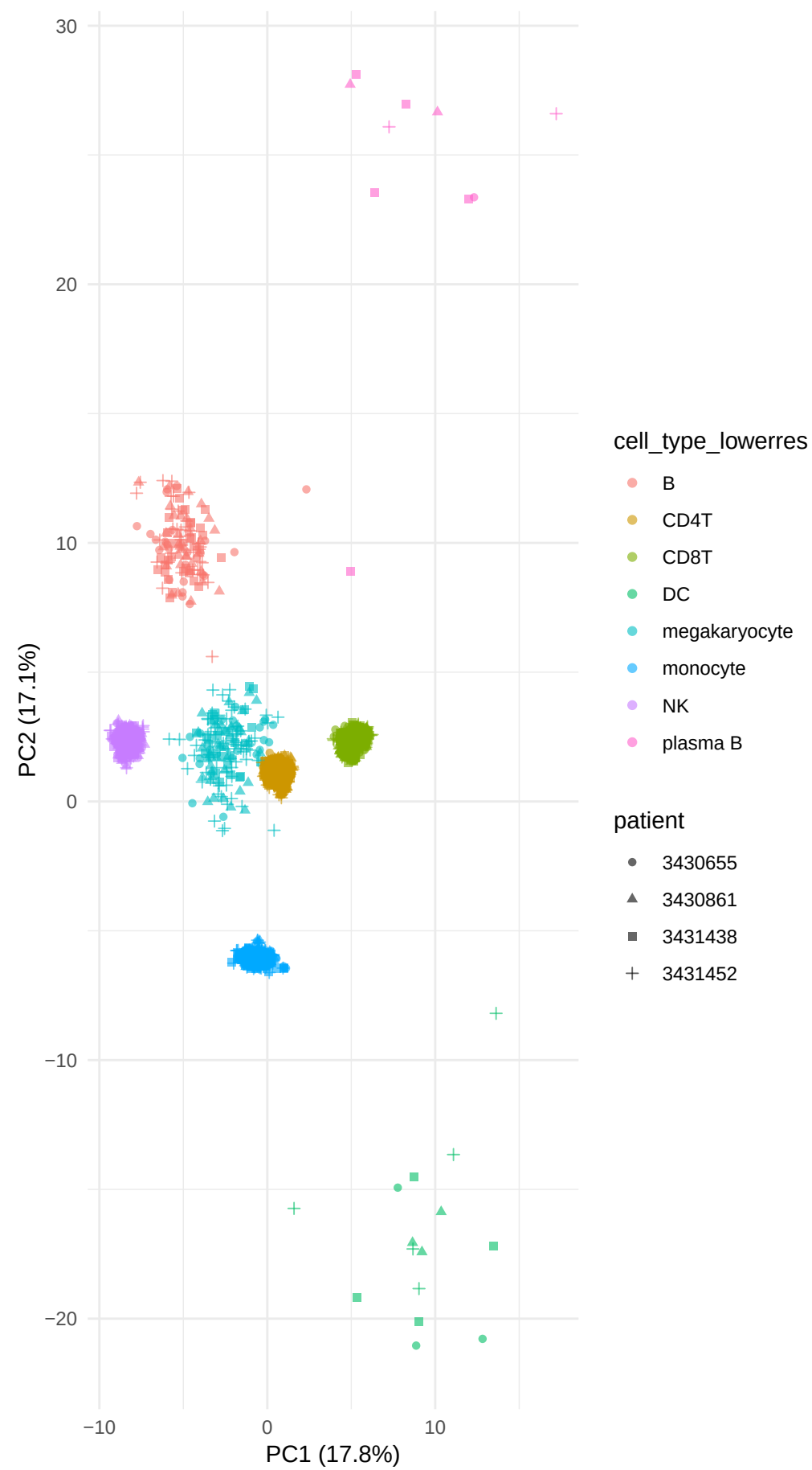
ASCA on cell_type_lowerres
