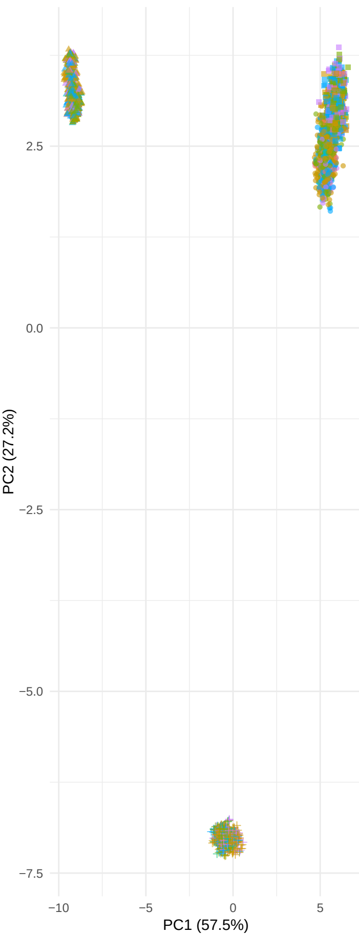
ASCA on patient
