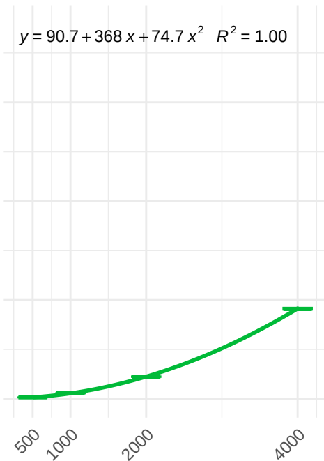
benchmarkFilterSamples
