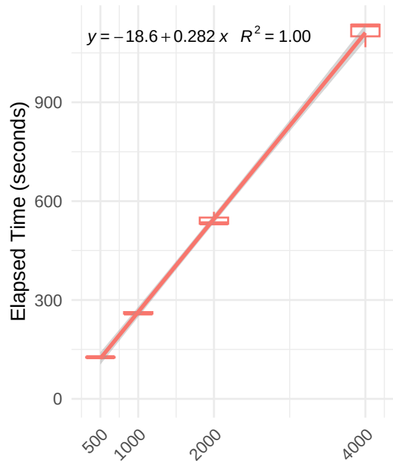
benchmarkAggPSM
