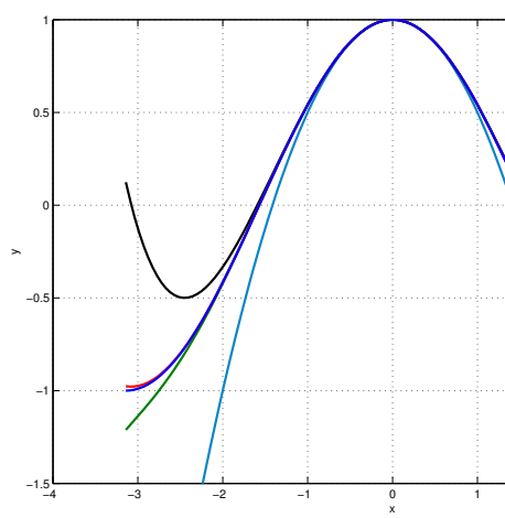
(a) \cos(x) , polinomios 2, 4, 6 y 8 grados (a) polynomials 2, 4, 6 and 8 degrees
