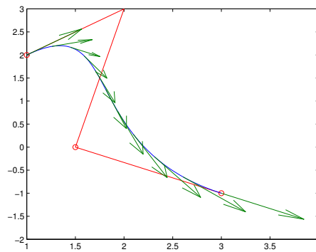
(a) Curva de Bézier (4 puntos) (a) Bézier's curve (4 points)
