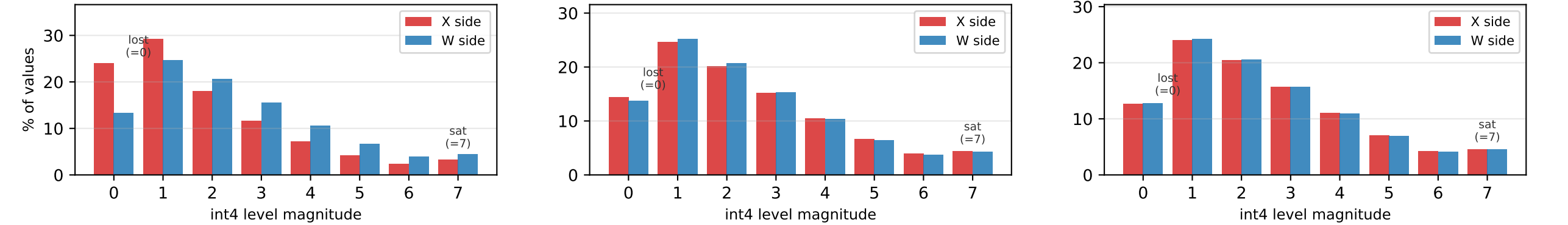
raw (no rotation) — level distribution (LLM.L02.gate_proj)
