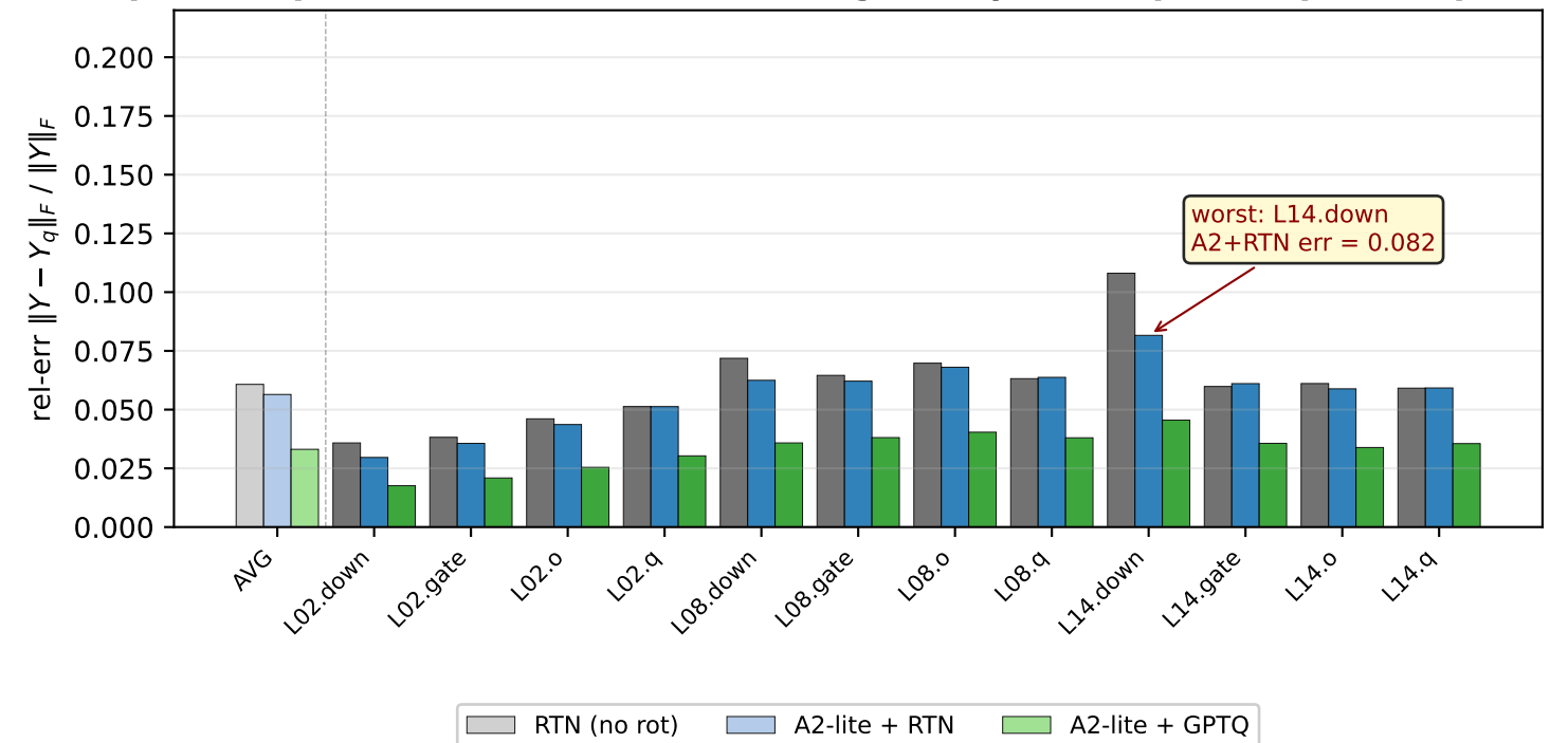
pi0.5 expert / action head — W4 weight-only rel-output-err per component
