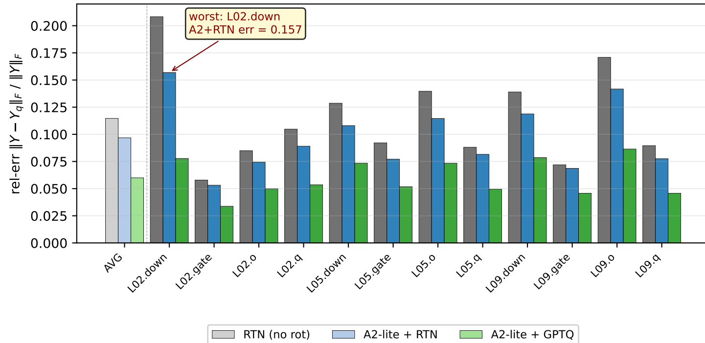
gr00t-N1.5 LLM (eagle) — W4 weight-only rel-output-err per component
