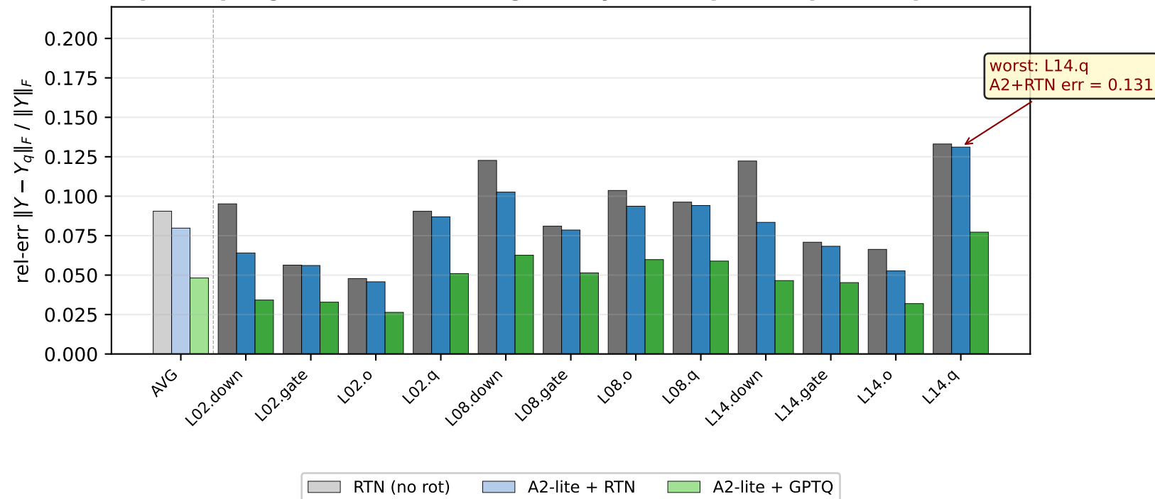
pi0.5 paligemma — W4 weight-only rel-output-err per component
