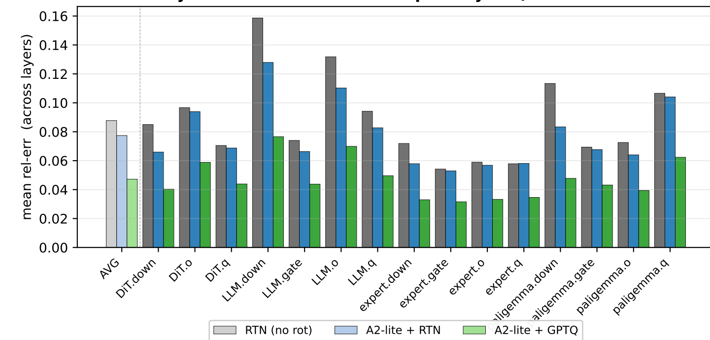
Per-kind summary: mean rel-err across sampled layers (AVG = mean over all kinds)
