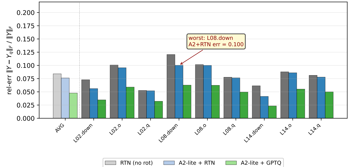
gr00t-N1.5 DiT — W4 weight-only rel-output-err per component
