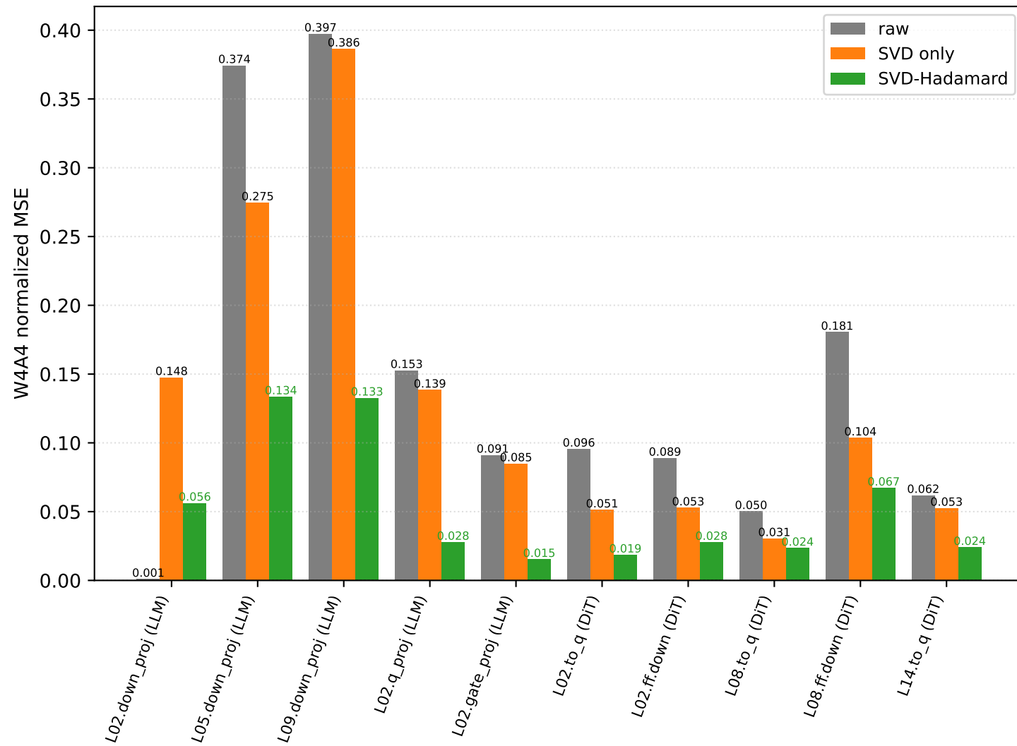
Layer-output quant MSE
