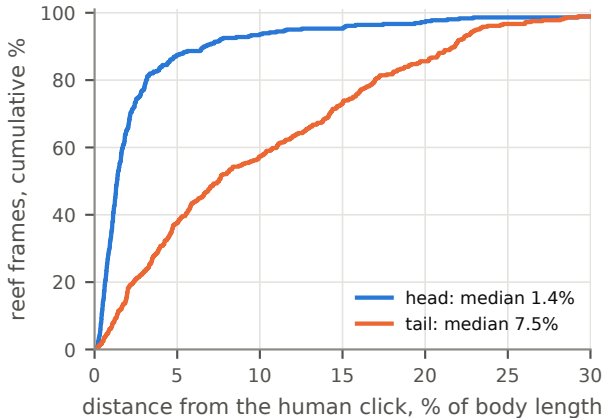
Automatic head and tail on reef fish (n=361)
