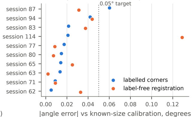
(b) every session, unknown object size
