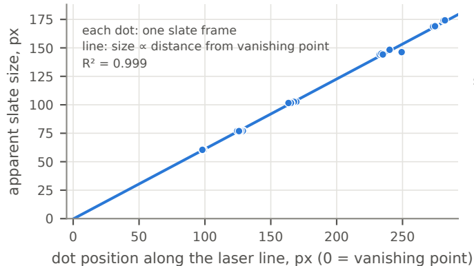
(a) one session: size shrinks to zero at the vanishing point
