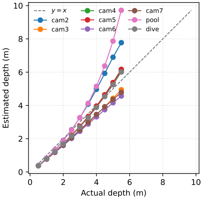
Pinhole-estimated depth under flat-port refraction
