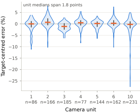
Percent length error by camera unit (repository only)
