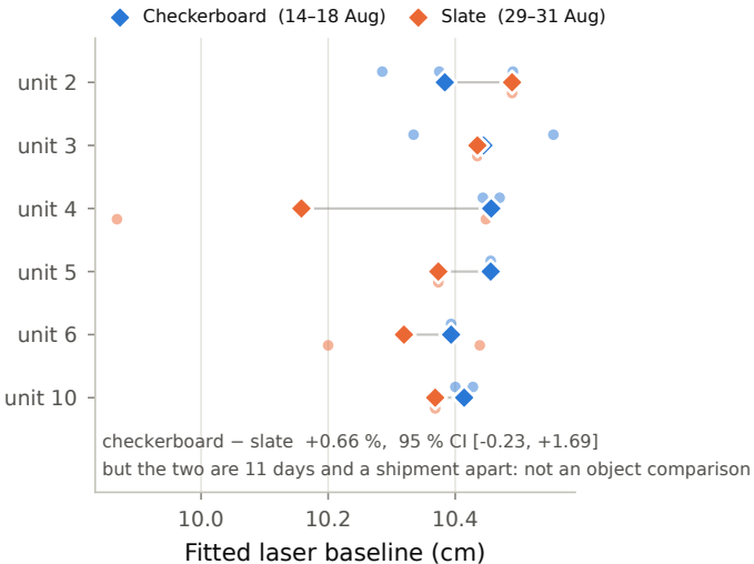
Laser baseline per unit, by calibration object and mount epoch
