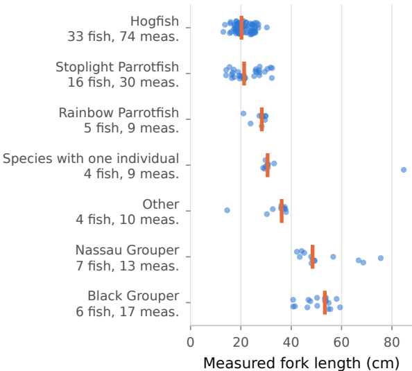
Measured fork length by species, seven deployments
