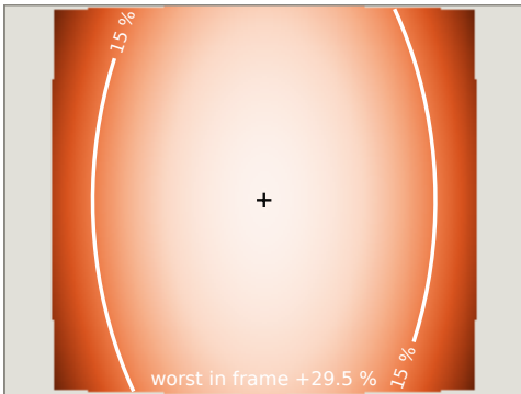
(a) Flat port, no corrective optic
