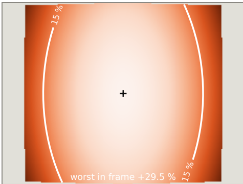
Flat port, no corrective optic
