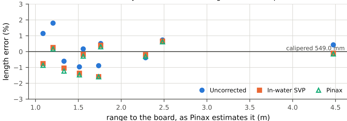
Camera-only end to end: measuring a 549.0 mm span
