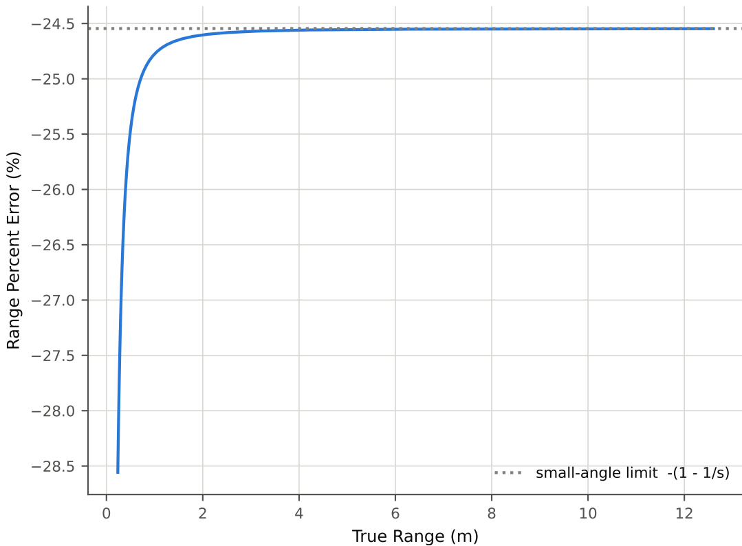
Range Error from an Uncorrected Angular Scale Error
