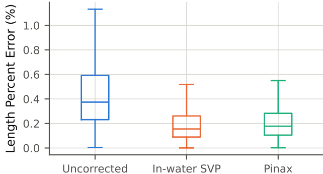
Local: distortion across a 295 mm span
