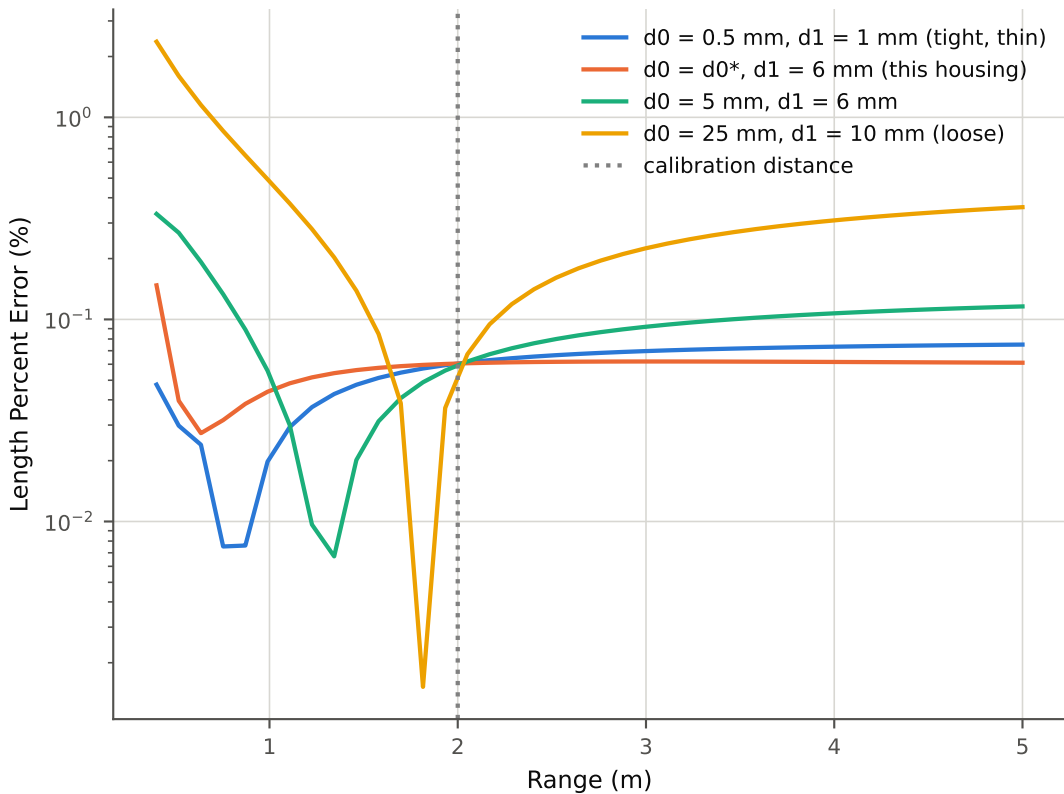
In-Water SVP Length Error vs Range, by Housing Geometry
