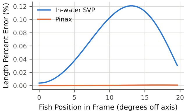
Length Error vs Field Position (corrected only)
