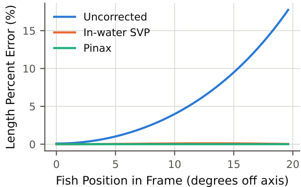
Length Error vs Field Position (0.3 m fish at 2.0 m)
