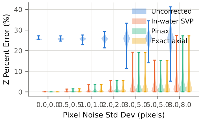
Range Error vs Pixel Noise (all pipelines)
