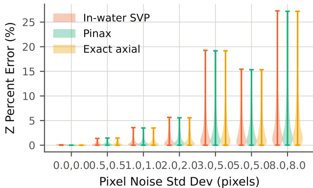
Range Error vs Pixel Noise (corrected only)
