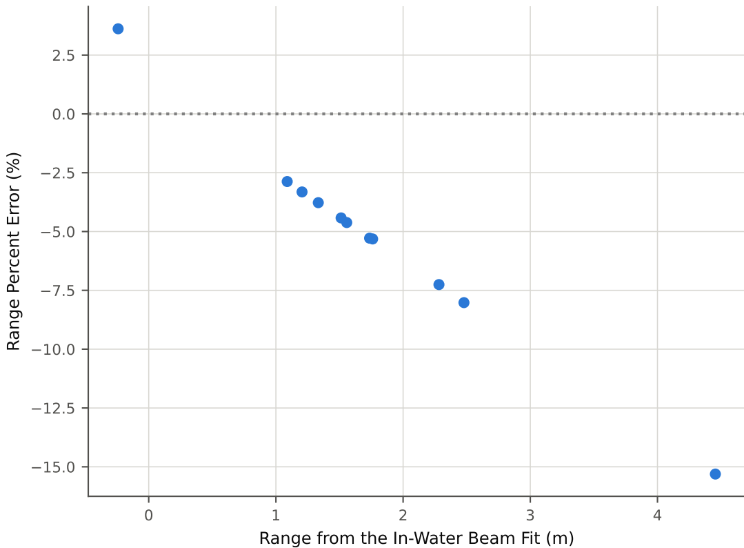
Range Error from Calibrating the Laser Dry
