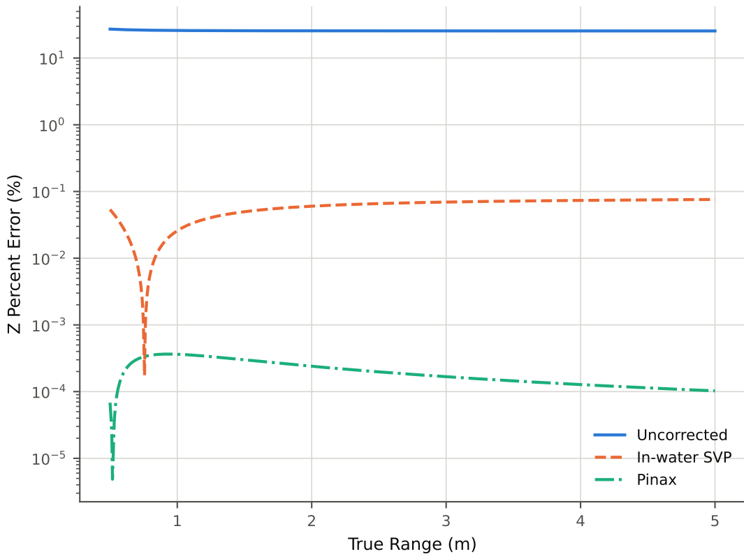
Range Error vs Distance (noise-free)
