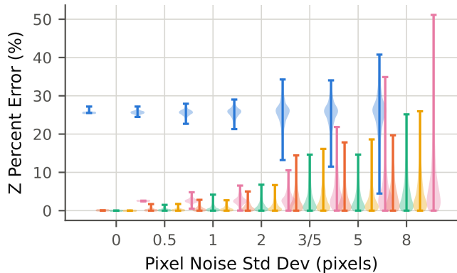
Uncorrected Pinax In-water SVP Exact axial Range Error vs Pixel Noise (all pipelines)
