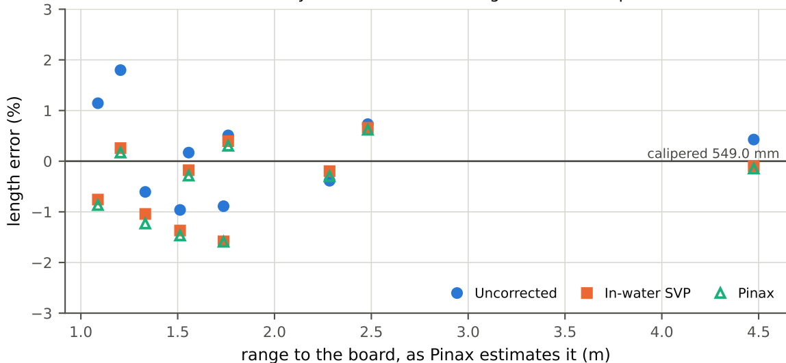
Camera-only end to end: measuring a 549.0 mm span
